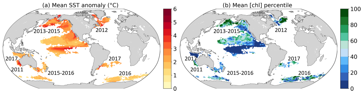
Figure 1. Recent (a) prominent large-scale marine heatwaves (MHWs) for which impacts have been documented and (b) associated changes in surface chlorophyll concentrations ([chl]). We use sea surface temperature (SST) and [chl] deseasonalized anomalies. MHWs are defined when SST anomalies exceed their percentile 99.5 locally, and numbers indicate the years of the MHW occurrences. (a) SST anomaly averaged over the MHW duration. (b) Percentile associated with the mean [chl] anomaly averaged over the duration of the MHW, compared to the local empirical distribution of [chl] daily anomalies from 1998 to 2018. The MHW extent is taken from Laufkötter et al. (2020) and corresponds to a spatiotemporally continuous area where each grid cell exhibits daily temperature anomalies above percentile 99.5.
