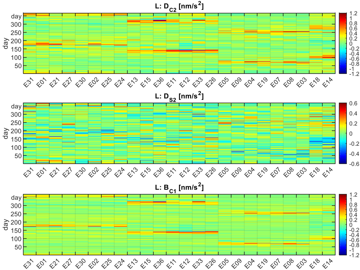
epoch-wise clocks
