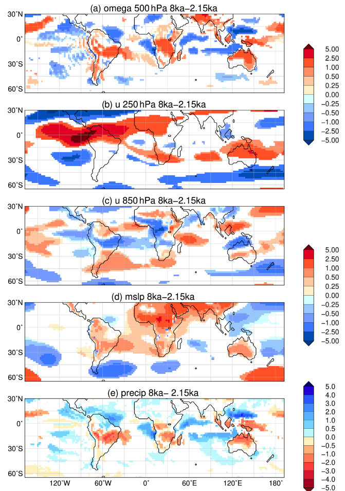
Figure 9. Simulated difference in December to February (DJF, austral summer) mean climate in the model for the time slice 8 ka compared to 2.15 ka, i.e. (a) vertical velocity ( \omega ) in 500 hPa ( 10^{-2} \text{ m s}^{-1} ) with blue colour showing increased uplift during 8 ka; (b) upper-tropospheric zonal wind ( u ) in 250 hPa ( \text{m s}^{-1} ) with blue colours indicating enhanced easterly wind; (c) low-level zonal flow ( u ) in 850 hPa ( \text{m s}^{-1} ); (d) mean sea level pressure (hPa) with low-pressure anomaly given in blue colours; and (e) mean seasonal precipitation ( \text{mm d}^{-1} ) with blue colours showing enhanced precipitation during 8 ka. Only significant changes are shown ( t test, 99 % confidence interval).
