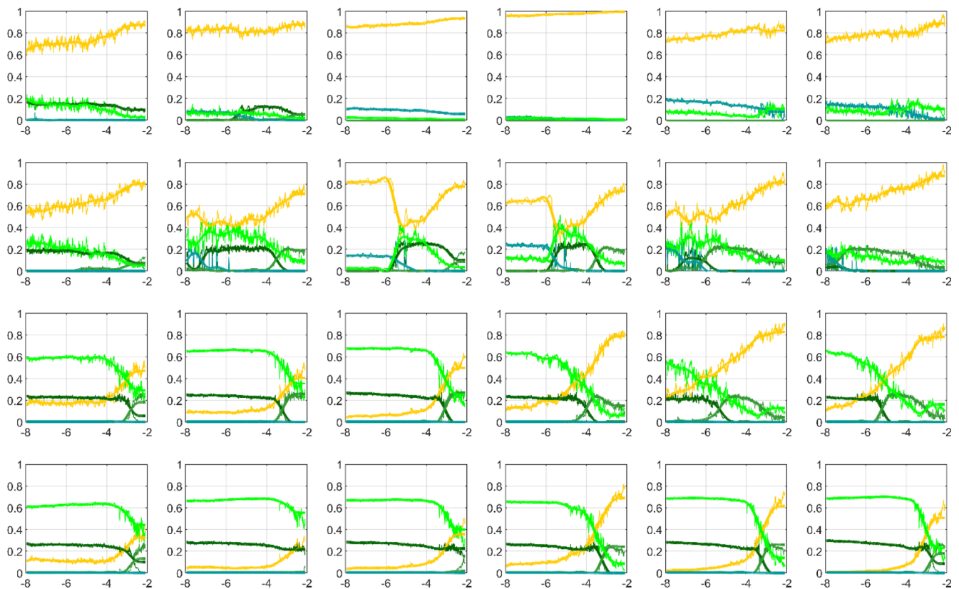
Figure 14. Simulated changes in PFTs in the today Sahara–Sahel region (part of region 3 in Fig. 12). The box in the upper left corner is centred at 25.18^{\circ} N, 15^{\circ} W, and the box in the lower right corner is at 19.59^{\circ} N, 5.63^{\circ} W. Like in Fig. 13, the fractional coverage V of PFTs in each grid cell is depicted as function of time, given as kyr b2k. The colours refer to bare soil fraction (yellow), grass (light green), tropical evergreen trees (dark green), tropical deciduous trees (green) and shrubs (blue).
