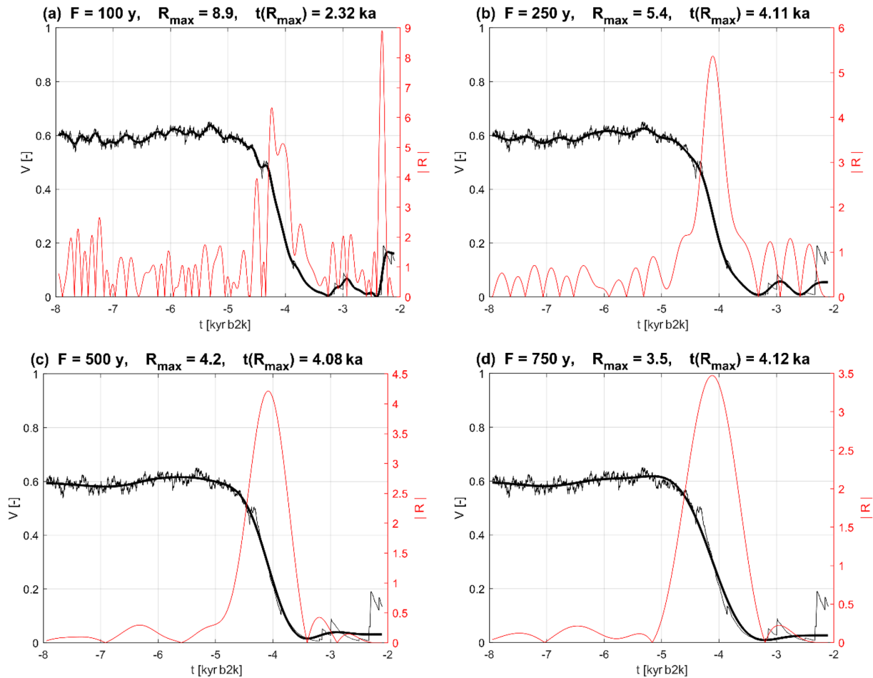
Figure C1. Effect of filtering on R_{\max} . Black lines indicate fractional coverage of extratropical deciduous trees in a grid box in East Siberia centred at 62.48^\circ\text{N} , 120^\circ\text{E} , in region 2 (see Figs. 12 and 13a) as function of time (in ka). The thin lines are annual values of fractional vegetation coverage V(t) , and the thick lines are filtered time series of V(t) using a Butterworth filter of the order of 5 with a low-pass filter of (a) F of 100 years, (b) F of 250 years, (c) F of 500 years, (d) F of 750 years. The absolute value of the relative change R is shown as a dotted red line. The titles of each subfigure indicate the strength of the low-pass filter F , the maximum of the absolute value of the relative change R_{\max} and the time t at which R_{\max} occurs.
