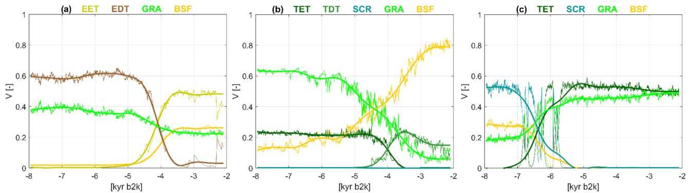
Figure 13. Examples of rapid transitions between simulated PFTs in a grid cell in (a) East Siberia (at the grid cell centred at 62.49^{\circ} N, 120^{\circ} E, in region 2 in Fig. 12), (b) today's Sahara–Sahel region (at 19.59^{\circ} N, 7.5^{\circ} W, in region 3) and (c) South Asia (at 19.59^{\circ} N, 78.75^{\circ} E, in region 4), shown as fractional coverage V(t) as function of time t , given as kyr b2k. The colours refer to different PFTs as indicated in the title line. EET: extratropical evergreen trees; EDT: extratropical deciduous trees; TET: tropical evergreen trees; TDT: tropical deciduous trees; SCR: shrubs; GRA: grass; BSF: bare soil fraction. The thin lines are annual values of fractional vegetation coverage, and the thick lines are filtered time series using a Butterworth filter of the order of 5 with a low-pass filter of 500 years.
