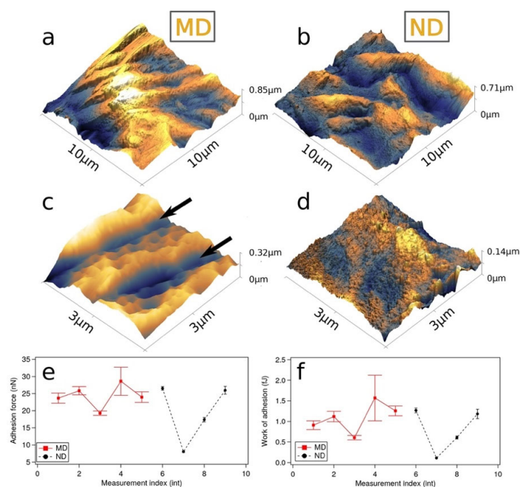
Figure 2. (a–d) AFM topography images of machined titanium samples (a,c) and \text{H}_2\text{SO}_4/\text{H}_2\text{O}_2 etched test object samples (b,d). 10 \mu\text{m} \times 10 \mu\text{m} images showed surface spanning between 102 and 157 nm. Higher magnification images show trenches (marked by arrows) due to the machining process for machined (c) surface. The adhesion force and work of adhesion between AFM tip and titanium surfaces are shown in (e,f). Both surfaces show similar adhesion forces (see text).
