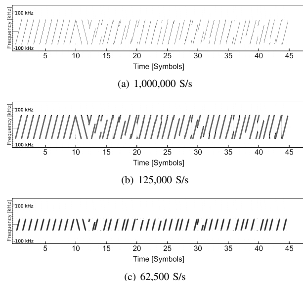
Fig. 13: The Effect of the LoRa Signal Sampling Rate
