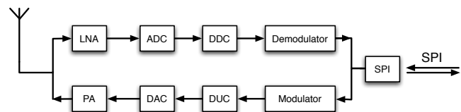
Fig. 3: LoRa Concentrator
