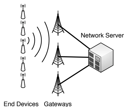
Fig. 1: LoRaWAN Architecture
