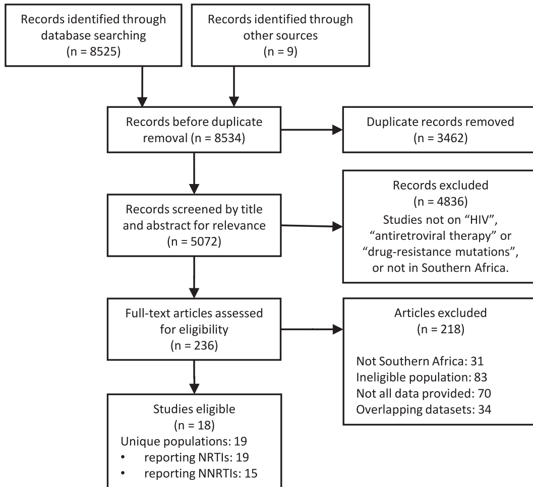
Fig. 2. PRISMA flow-chart of inclusion of studies and populations in the systematic review.
