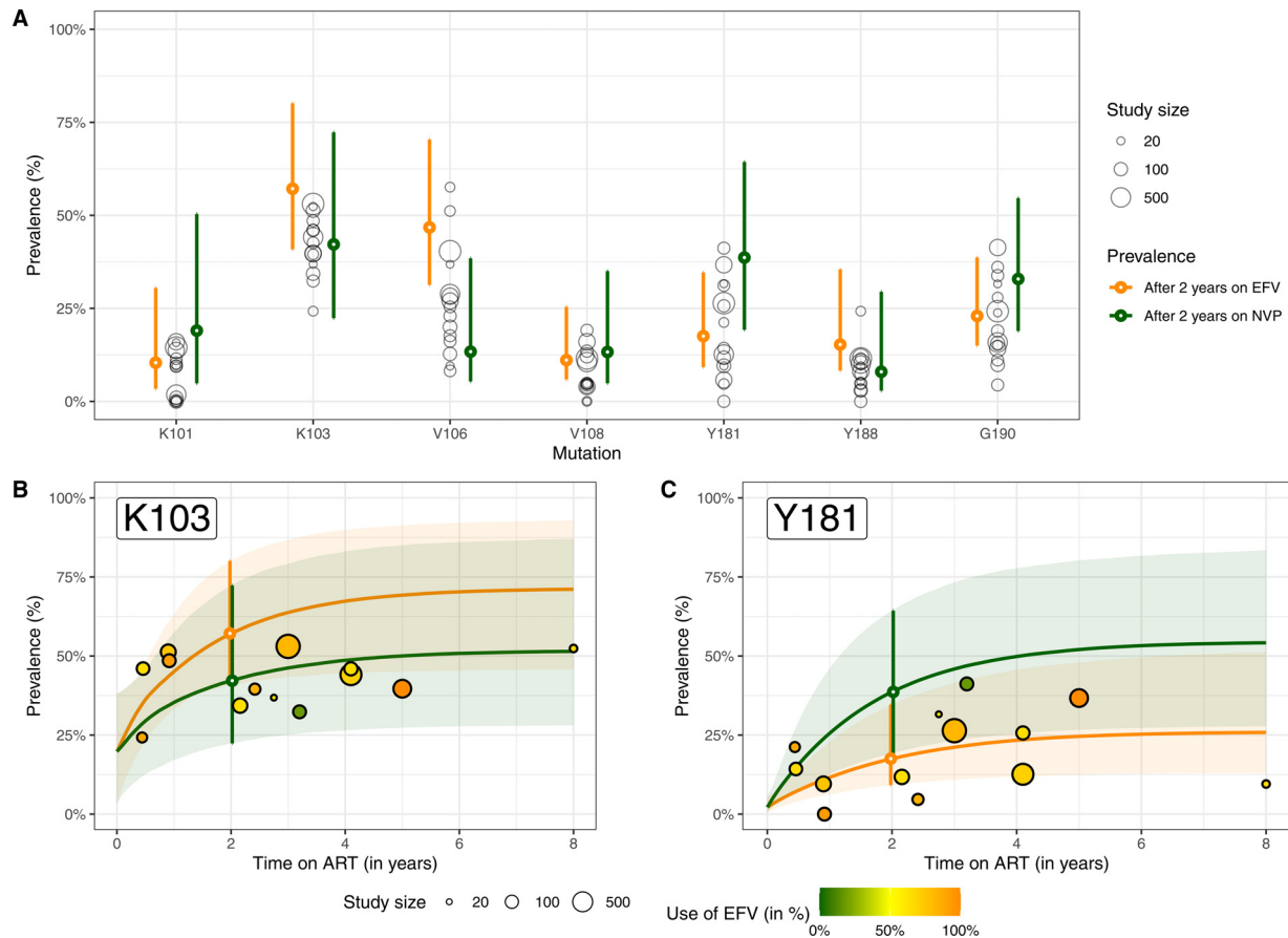
Fig. 4. Prevalence of seven NNRTI drug resistance mutations. Panel A: Prevalences after 2 years on either EFV- or NVP-based regimen. Panel B: Prevalence of the K103 mutation over time. Panel C: Prevalence of the Y181 mutation over time. Points and vertical lines: median and 95% credibility intervals of baseline prevalence (black), prevalence after 2 years on EFV (orange) or NVP (green). Shaded area: 95% credibility interval over time. In contrast to Fig. 3, the Panel A does not report baseline prevalence because EFV and NVP select for the same NNRTI DRMs, which prevents the model from providing reliable estimates (For interpretation of the references to color in this figure legend, the reader is referred to the Web version of this article.)
