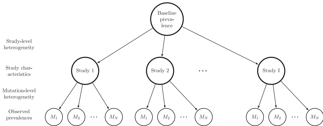
Fig. 1. Bayesian hierarchical model adjusting for the different levels of heterogeneity.
