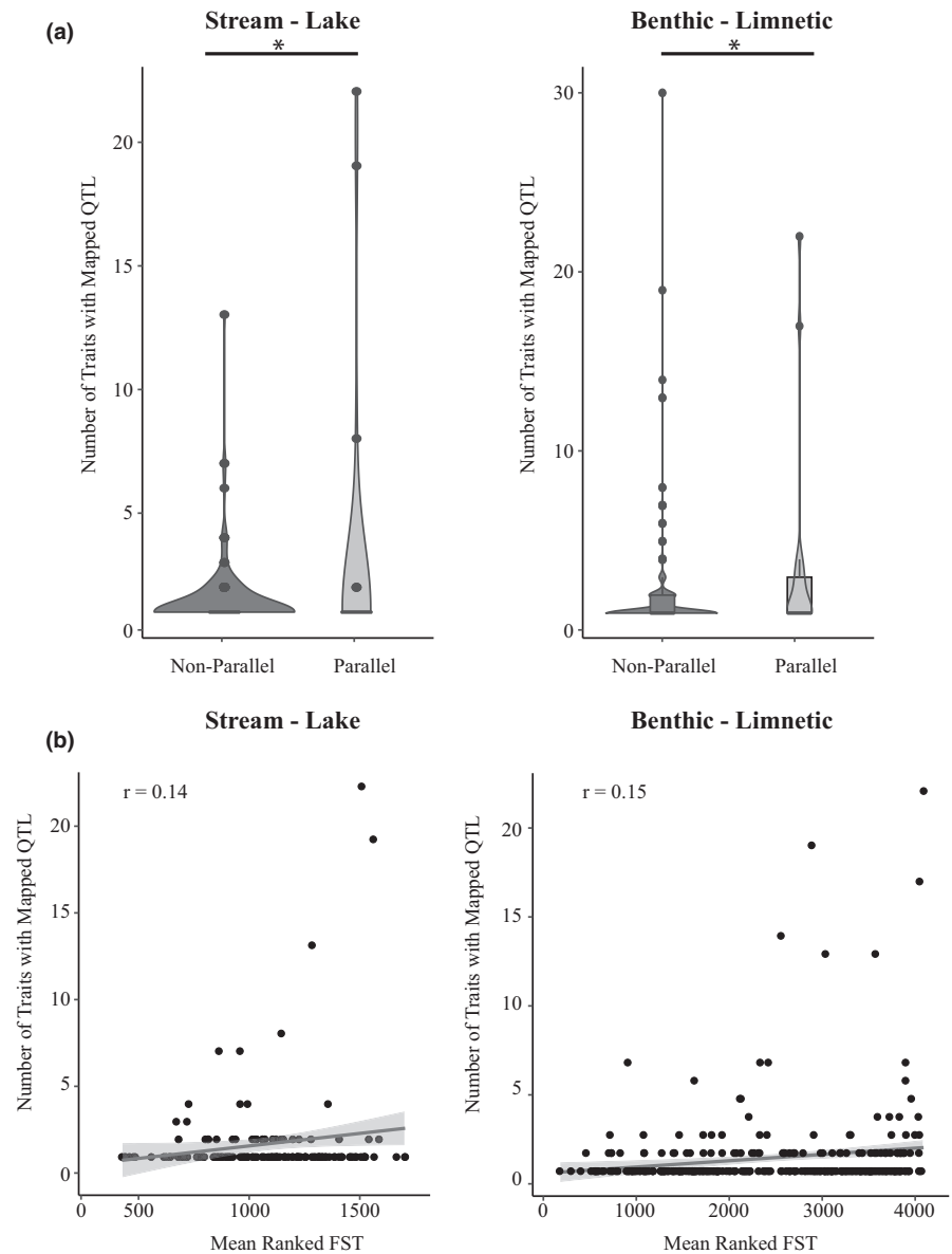
FIGURE 1 (a) Comparisons of pleiotropy (number of traits with mapped QTL) between parallel and nonparallel windows. An asterisk indicates permutation test p < .05 . (b) Relationship between pleiotropy (number of traits with mapped QTL) and mean F_{ST} rank. Note that the total number of windows with data or having unique F_{ST} values differed between the stream-lake and benthic-limnetic ecotype pairs so that the mean F_{ST} rank values differ among these comparisons
