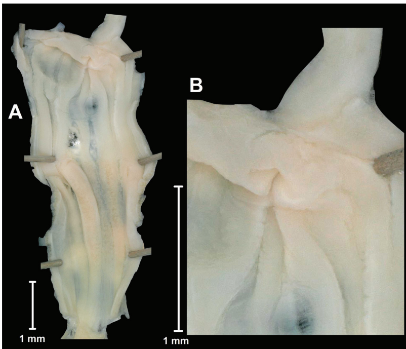
Figure 4. Inner wall of the penis of Bouchetcamaena platytropis Möllendorff, 1894 (ZMH 51934) A entire penis B penis-epiphallus transition.
