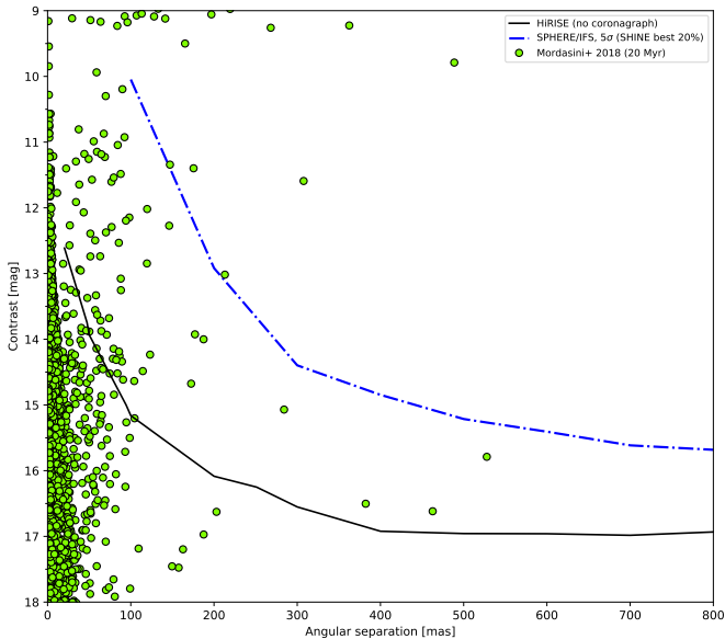
Fig. 12. Detection limits of 5\sigma for HiRISE derived in the present work for a bright nearby young star ( H = 3.5 , 19 pc, 20 Myr), compared to the 20% best SPHERE/SHINE detection limits. We overplot state-of-the-art population synthesis models based on the core accretion formation scenario (Mordasini 2018; Emsenhuber et al. 2020a,b).
