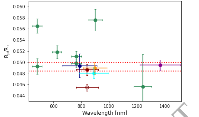
Figure 12. Planet-star radius ratio as a function of wavelength for GJ 1132 b. Points are colour-coded as follows: blue – CHEOPS , red – MEarth, orange – Diamond-Lowe et al. (2018), green – Southworth et al. (2017), magenta – WFC3, cyan – TESS. The radius ratio obtained from Spitzer observations at 4.5\ \mu\text{m} is indicated with dotted lines. The planet-star radius ratio measured using MEarth data by Dittmann et al. (2017) is plotted with an open circle symbol.
