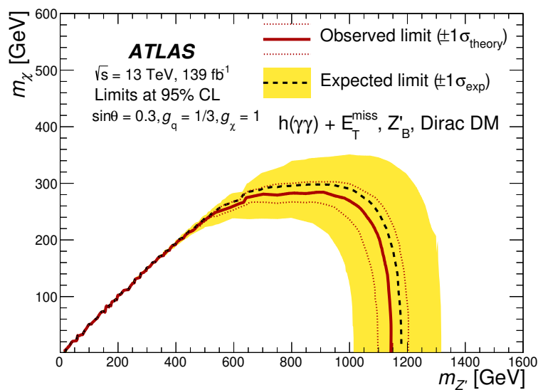
Figure 7. The observed (solid line) and expected (dashed lines) exclusion limit contours at 95% CL for the Z'_B model in the m_\chi - m_{Z'} plane, for \sin\theta = 0.3 , g_q = 1/3 , and g_\chi = 1 . The dotted lines represent the \pm 1\sigma theoretical uncertainty for the observed limit. The \pm 1\sigma expected exclusion limit contour is shown as the yellow band.
