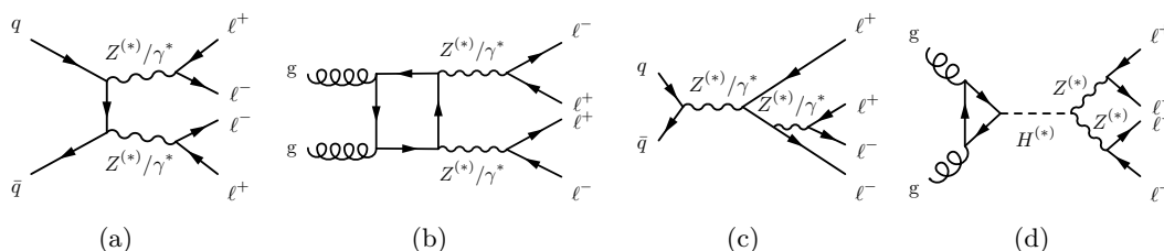
Figure 1. Main contributions to the pp \rightarrow 4\ell (\ell = e, \mu) process: (a) t -channel q\bar{q} \rightarrow 4\ell production, (b) gluon-induced gg \rightarrow 4\ell production via a quark loop, (c) internal conversion in Z boson decays and (d) Higgs-boson-mediated s -channel production (here: gluon-gluon fusion). The superscript (*) refers to a particle that can be either on-shell or off-shell, whereas \ast indicates that it is always off-shell.
