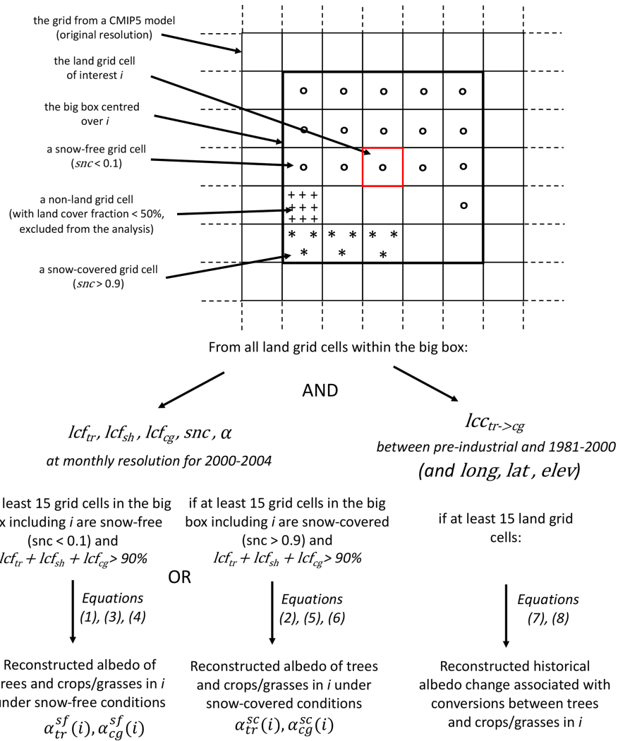
Figure 1. Description of the two employed reconstruction methodologies; snc stands for snow cover fraction, \alpha for albedo, lcf for land cover fraction, and lcc for land cover conversion. The suffixes tr, sh, and cg stand for trees, shrubs, and crops–grasses, respectively, with long for longitude, lat for latitude, and elev for elevation.
