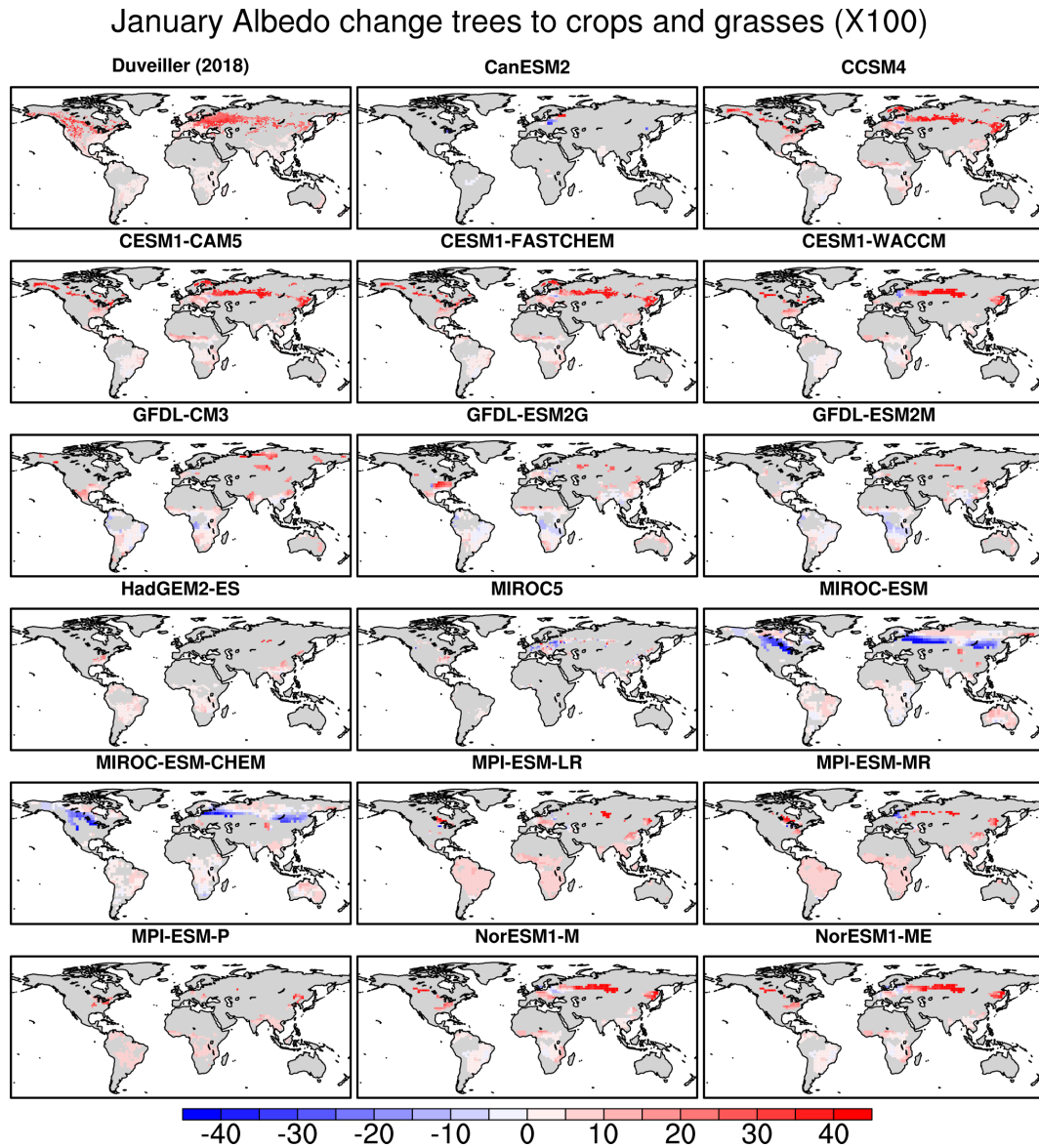
Figure 11. Same as Fig. 10, but for January. Note that the scale is different.
