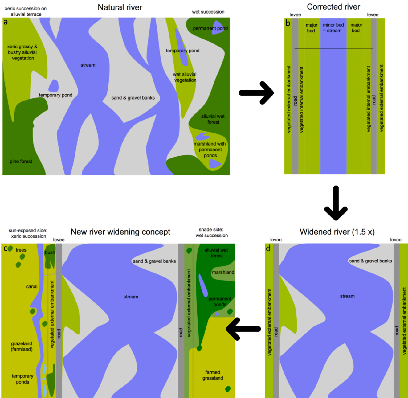
Fig. 1. Own schematic representation of (a) a natural river, (b) a conventionally corrected river, (c) a river widened by a factor 1.5 with additional buffer zones outside the levees, (d) a river restored with today's standard of widening the bed by a factor 1.5 without a buffer zone. C illustrates the integrated concept of river restoration developed in this study.
