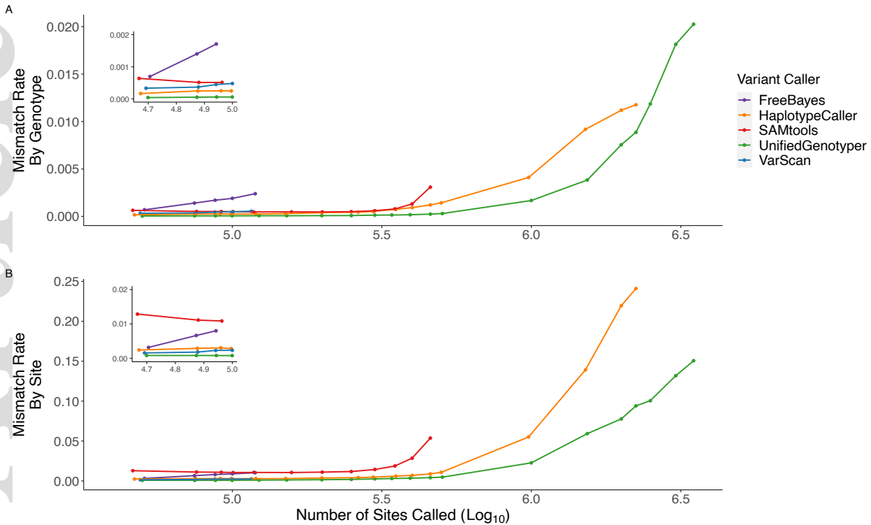
Fig. 2: Comparison of mismatch rates by genotype (A) and by site (B) between variant callers at variable numbers of sites called. Mismatch rates were calculated as the proportion of mismatched parent-offspring genotype calls out of the total number of genotypes called (A) and as the proportion of sites with at least one mismatched parent-offspring genotype call out of the total number of sites (B). Inset plots show a magnification of the mismatch rates over 50k to 100k sites called. Variation in the number of sites called for a particular variant caller was generated by additional incremental filtering to different degrees with depth, genotype quality, and quality score where applicable.
