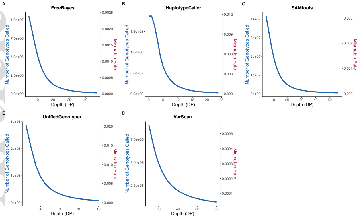
Fig. 3: Effect of filtering by depth (DP) on the number of genotypes called (blue) and the genotype mismatch rates (red) after baseline filtering. Note: Scales differ on all three axes for each panel.
