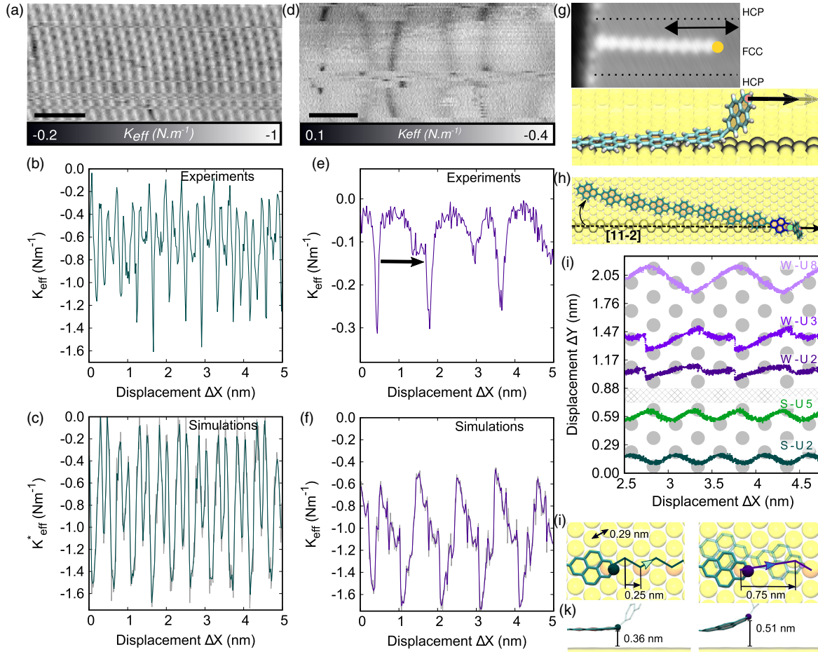
FIG. 1. Slithering dynamics of a deca-pyrenylene on Au(111). Experimental stiffness maps k_{\text{eff}}(x, y) (a),(d) representative trace (b),(e) and corresponding simulation results (c),(f) obtained during the sliding at different heights, i.e., in strong contact (a)–(c) and in a weak contact (d)–(f) regimes. (g) Initial configuration of the polymer before sliding, and schematic side view representation. (h) Representative configuration of the deca-pyrenylene during sliding. (i) Paracarbon atom trajectory of the second and fifth units for the strong contact regime (S-U2, S-U5 shown in green) and trajectories of the second, third, and eighth units for the weak contact regime (W-U2, W-U3, W-U8 shown in purple). Top (j) and side (k) views of intermediate sliding stages in the strong (left) and weak (right) contact regimes.
