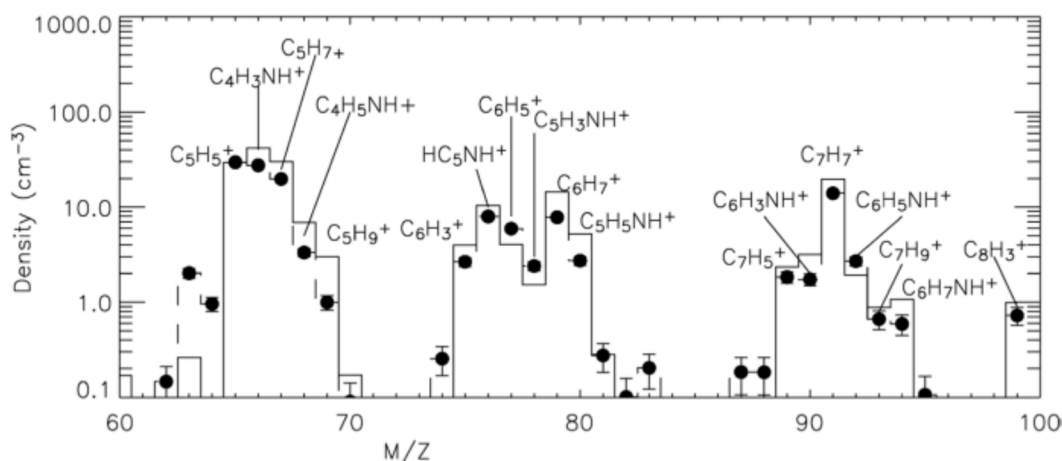
Fig. 6 Cassini observation of ionospheric heavy ions [46]
