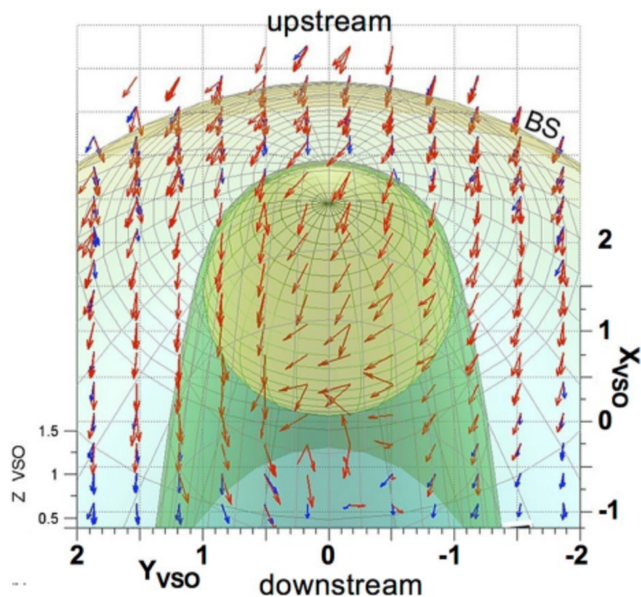
Fig. 4 Ion convection directions observed by Venus Express [36]
