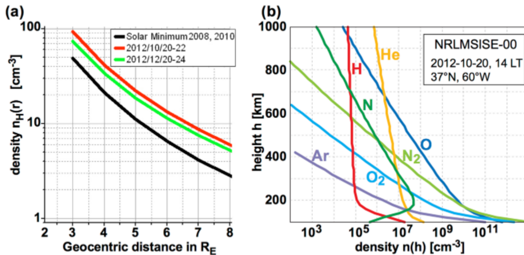
Fig. 1 a Average exospheric hydrogen density profile that is model-fitted from Lyman-alpha line-of-sight observations by the two TWINS spacecraft [20]. b Example altitude profile by the International MSIS model ( https://ccmc.gsfc.nasa.gov/modelweb/models/nrlmsise00.php ). The smoothness of the profile (nearly exponential above 200 km for neutral species) comes from the lack of observations beyond the 1960's [21]
