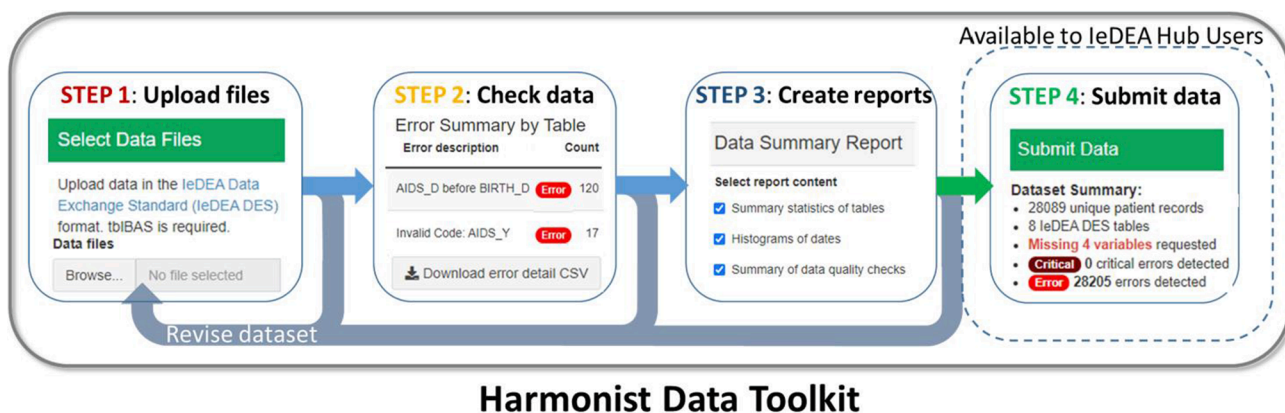
Fig. 6. Harmonist Data Toolkit workflow overview.
