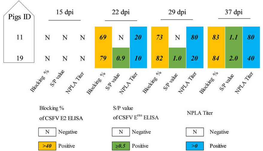
FIG 5 Evaluation of the humoral immune response in piglets after vPDR-H 30 K-5U infection. The E2- and E ms -specific antibody responses were measured by specific ELISAs and are shown as percent blocking or as S/P ratios. The neutralizing antibody titers were determined by the NPLA at weekly intervals. The cutoff values for positive samples are indicated for the respective test.
