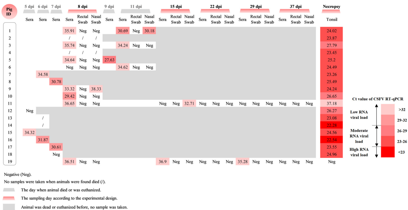
FIG 4 CSFV RNA detection in sera, swabs, and tonsils from the piglets infected with vPDR-H 30 K-5U. The CSFV RNA levels were determined by RT-qPCR in the sera and swabs at the indicated sampling time points and in the tonsils obtained at necropsy. C T values above 40 were considered negative.
