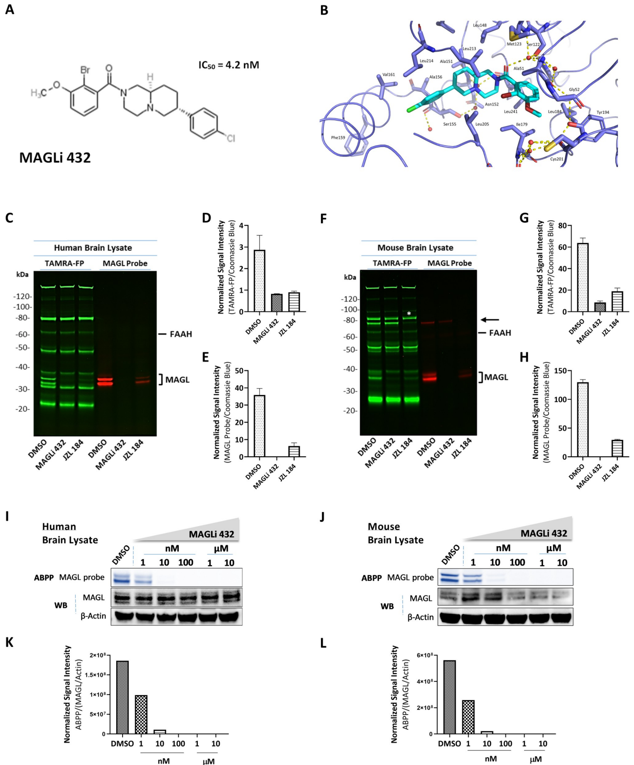
Fig 1. MAGLi 432 blocks MAGL in human and mouse brain lysates in a selective and potent manner. (A) Chemical structure of MAGLi 432 with an IC_{50} = 4.2 \text{ nM} in human MAGL as determined by enzymatic assays. (B) X-ray co-crystal structure of MAGLi 432 (cyan) with human MAGL (blue). View of the active site of human MAGL (blue) reveals a non-covalent binding of the inhibitor. Interactions of MAGLi 432 with the catalytic Ser122 are mediated through the amide carbonyl group via a water molecule located in the oxyanion hole. Hydrogen bonds are depicted as yellow dashed lines.
