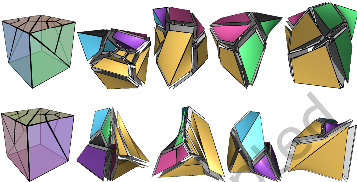
Fig. 24. The set of the hexahedrizations of the buffer cubes that the [Erickson 2014]’s algorithm uses to mesh arbitrary domains. (top) Cells with 20 quadrilaterals are meshed with 37 hexahedra. (bottom) Cells with 22 quadrilaterals are meshed with 40 hexahedra. Elements are colour coded to show the different sides of the original cubes (top-left and bottom-left). Image from [Verhetsel et al. 2019b].
