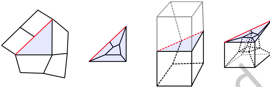
Fig. 15. If a quad maps two of its four edges onto a linear feature line it becomes locally degenerate (left). Splitting it into 5 sub-quads ensures enough degrees of freedom to produce all valid mesh elements. Similar configurations may also occur on 3D meshes, and can be resolved with a special padding scheme that splits a hexahedron into 6 sub elements (right). Image from [Gao et al. 2019].
