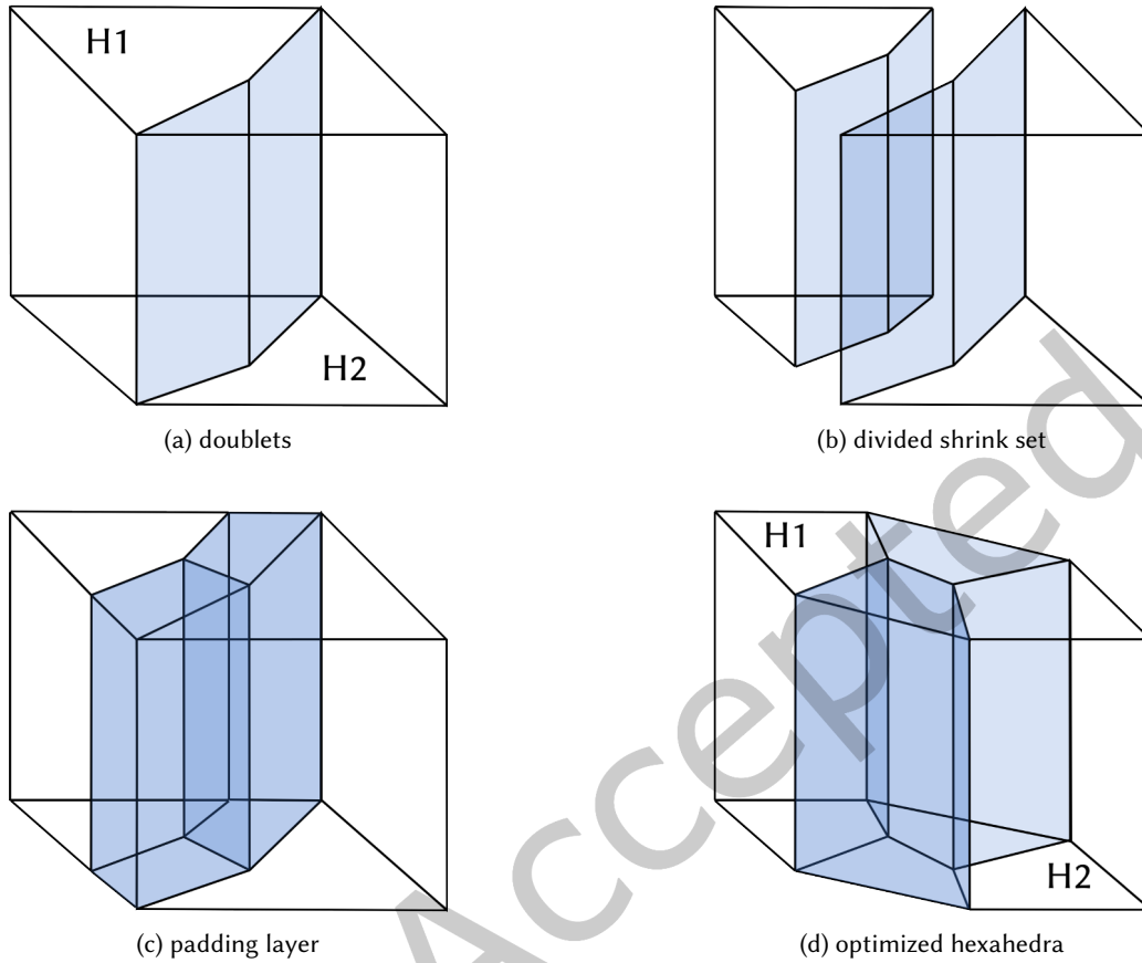
Fig. 25. A summary of the padding pipeline: (a) The hexahedra H1 and H2 share two faces forming two doublets. (b) The shrink set is disconnected to the other elements in the mesh. (c) The elements of the shrink set are linked to the mesh forming the padding layer. (d) The hexahedra involved in the refinement can now be optimized with a smoothing/untangling step.
