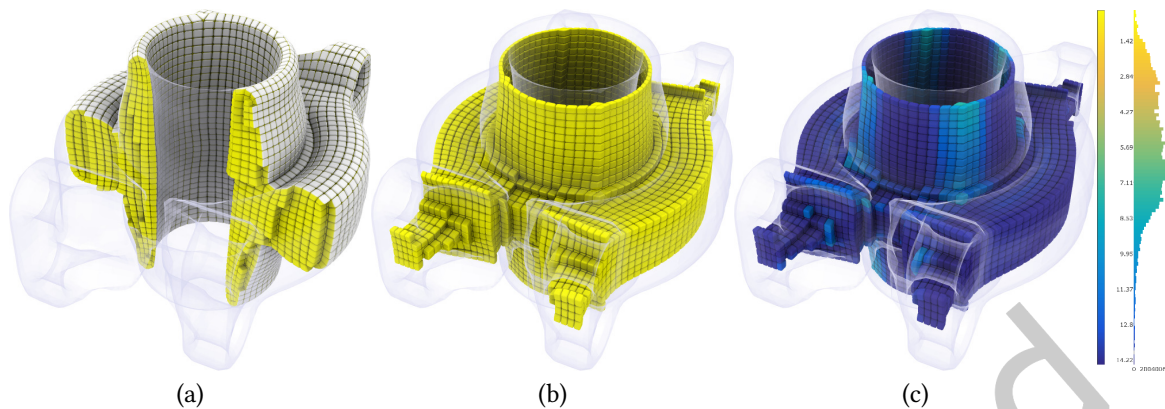
Fig. 33. The interactive visualization tools offered by Hexalab: Internal exploration using a sweeping plane (a) or the peeling tool (b); Coloring elements by their quality and the resulting histogram (c).
