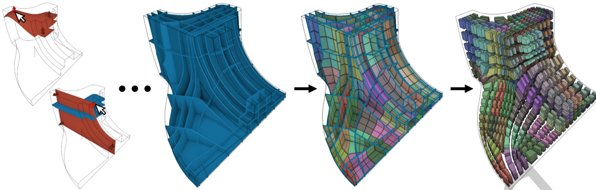
Fig. 10. Interactive sheet-based hex-mesh modeling. Image from [Takayama 2019].
