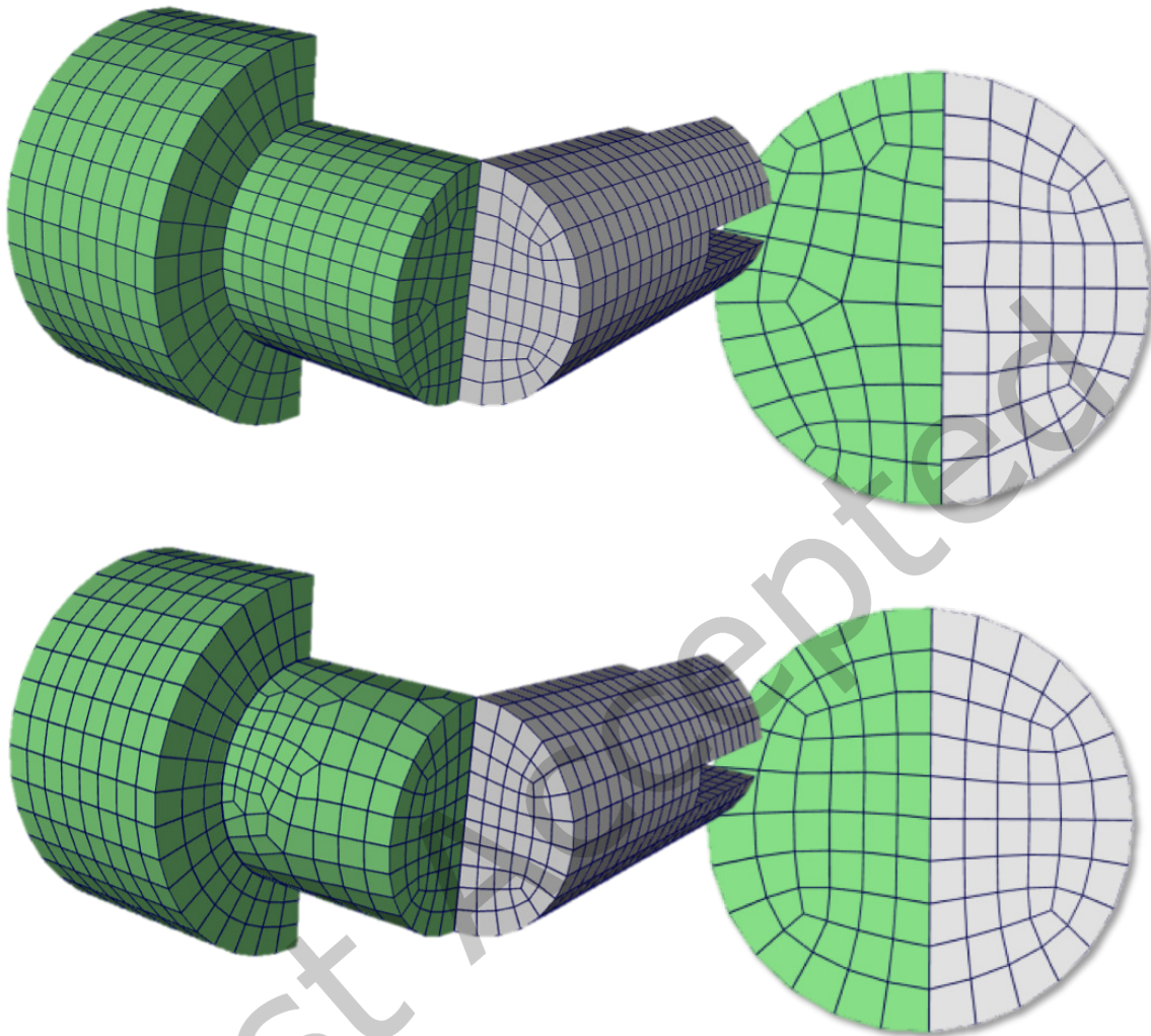
Fig. 23. Two meshes generated using sweeping are not conform along a contact surface (top); Performing sheet operations on the green mesh allows to get a conforming interface (bottom). Image from [Staten et al. 2010b].
