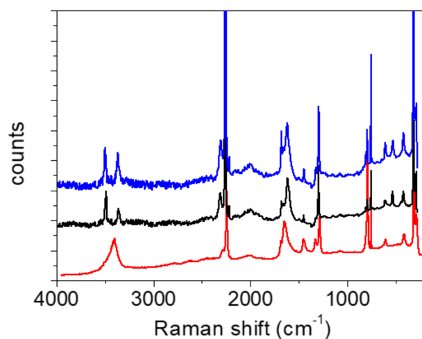
Figure 6. The Raman spectrum of ADAD, recorded at T = 25\text{ °C} (red line), T = -130\text{ °C} (black line), and T = -160\text{ °C} (blue line). Spectra were recorded with 585 nm laser.
