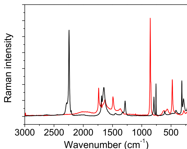
Figure 11. FT Raman spectra of oxalic acid dihydrate (red line) and acetylenedicarboxylic acid dihydrate (black line).
