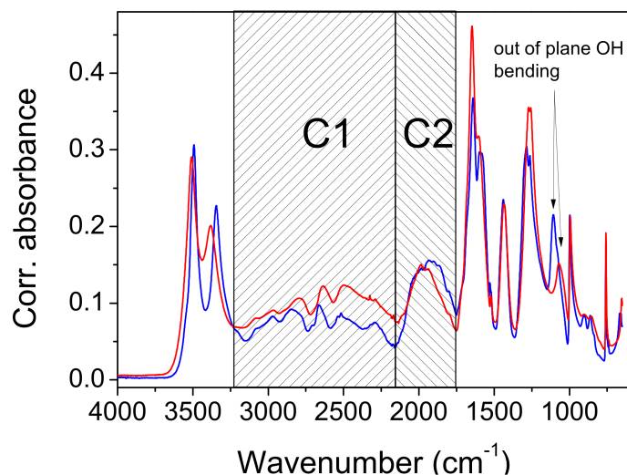
Figure 4. The infrared spectrum of ADAD recorded at T = 25\text{ }^\circ\text{C} (red line) and T = -150\text{ }^\circ\text{C} (blue line). C1 and C2 represent high- and low-frequency regions of the broad OH stretch, respectively.
