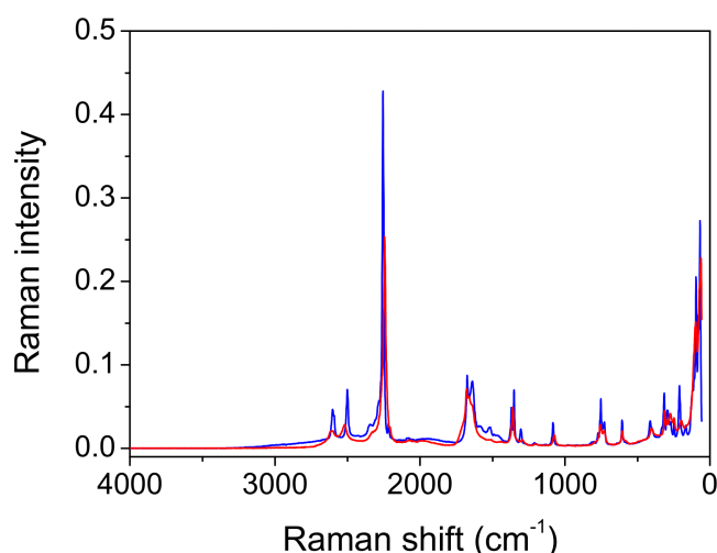
Figure 7. FT-Raman spectrum of ADAD (deuterated), recorded at T = 25\text{ °C} (red line) and T = -110\text{ °C} (blue line). FT-Raman spectrum of ADAD (protic) is presented in SI (Figure S4).
