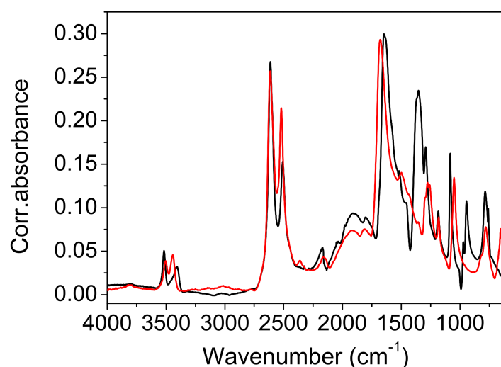
Figure 10. ATR spectra of deuterated oxalic acid dihydrate (red line) and deuterated acetylenedicarboxylic acid dihydrate (black line).
