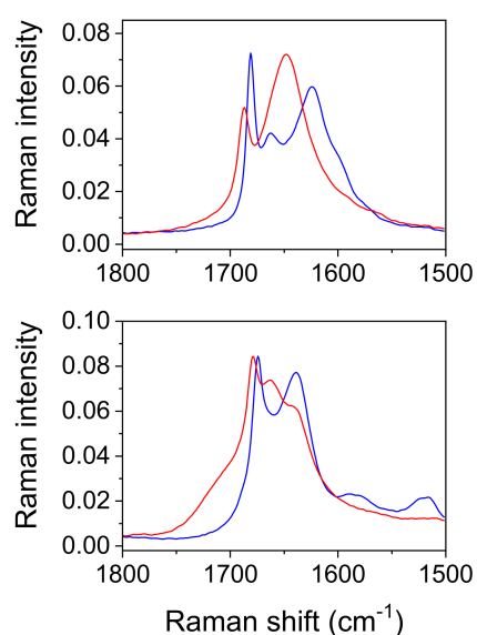
Figure 8. Enlarged region of carboxylate stretching vibration in FT Raman spectra of ADAD. Red spectra are recorded at room temperature, and blue at -110 °C. ( Upper graph ): protiated ADAD, ( bottom graph ): deuterated ADAD; spectra are scaled to same intensity.
