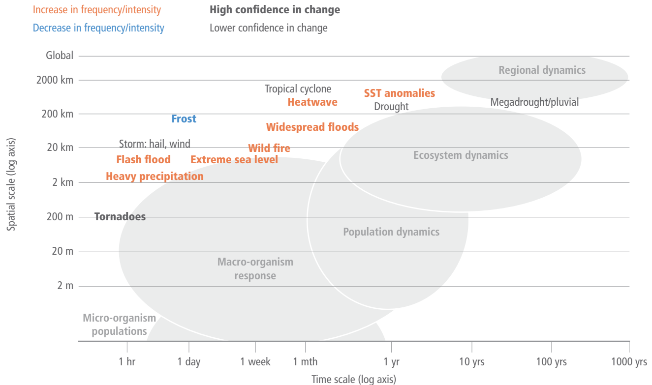
Figure 2.3 | Spatial and temporal scales of typical extreme weather and climate events and the biological systems they impact (shaded grey). Individuals, populations and ecosystems within these space-time ranges respond to relevant climate stressors. Orange (blue) labels indicate an increase (decrease) in the frequency or intensity of the event, with bold font reflecting confidence in the change. Non-bold black labels indicate low confidence in observed changes in frequency or intensity of these events. Each event type indicated in the figure is likely to affect biological systems at all temporal and spatial scales located to the left and below the specific event position in the figure. From Ummenhofer and Meehl (2017).
