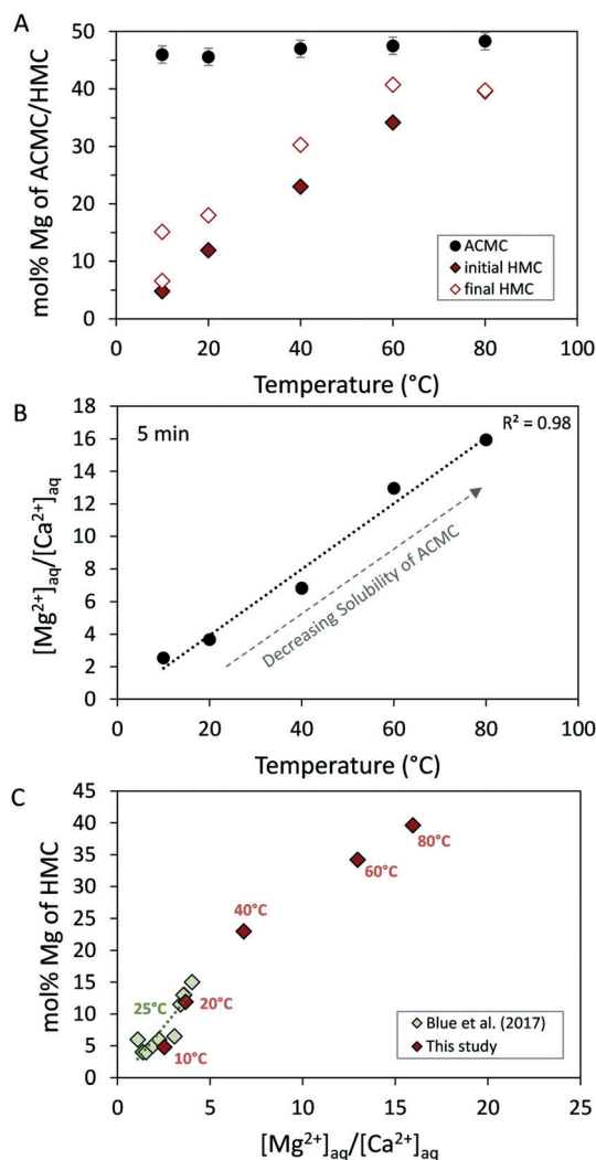
Fig. 5 (A) Temperature of the solution versus the Mg content of (i) ACMC obtained at 0.3 min of reaction time ( [Mg]_{\text{solid}} values in Table 2), (ii) initial HMC obtained at 21 min in experiment T_{10} °C and 11 min in experiments performed at \geq 20 °C and (iii) final HMC obtained at 1 day of reaction time. Note here that the Mg contents of HMCs were calculated from the d_{104} values of calcite XRD peaks ( [Mg]_{\text{XRD}} values in Table 1), whereas the Mg content of ACMC was calculated from solid digestion ( [Mg]_{\text{solid}} values in Table 2). (B) Temperature of the solution versus the Mg^{2+}/Ca^{2+} ratio of the solution at 5 min of reaction time (Table S2 † ). (C) Mg^{2+}/Ca^{2+} ratio of the solution at 5 min versus the Mg content of (i) initial HMC from this study, of initial HMC from experiments conducted at stirred conditions reported by Blue et al. 51
