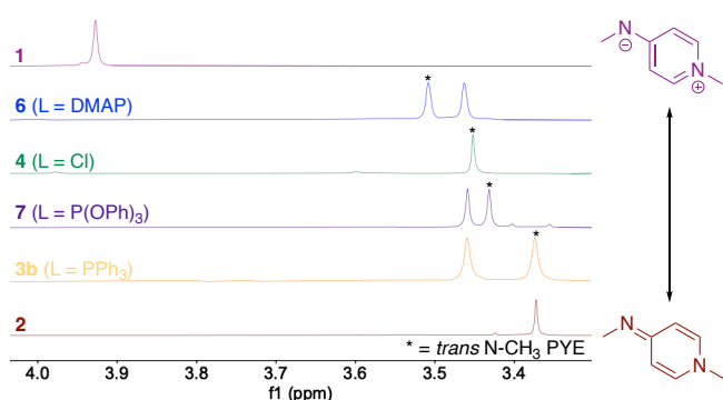
Figure 3. ^1\text{H} NMR spectra ( \text{CD}_2\text{Cl}_2 , 300 MHz) of 1 and 2 , and complexes 3b , 4 , 6 and 7 ( trans refers to \text{N}-\text{CH}_3 group of the PYE site trans to ancillary ligand L).
