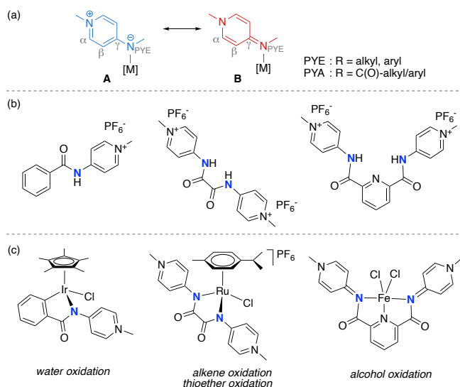
Figure 1. (a) Limiting resonance structures of PYA/PYE ligands featuring an anionic or a neutral coordination site; (b) examples of mono-, bi-, and tri-dentate PYA/PYE ligand precursors; (c) representative PYA complexes with catalytic activity.
