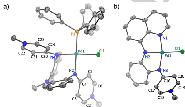
Figure 5. ORTEP representation of 10 (a) and 12 (b) at 50% probability level (all hydrogen atoms and BPh 4 anion of 10 omitted, rings below the coordination plane in lighter shade). Selected bond distances (Å) and bond angles (deg) for complex 10 : Pd1–Cl1 2.3076(3), Pd1–P1 2.2703(3), Pd1–N2 2.0724(10), Pd1–N4 2.0274(10), N4–C19 1.4227(14), N2–C7 1.4182(15), N4–C20 1.3221(15),
