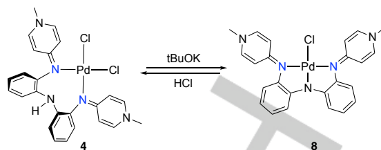
Scheme 3. Xantphos-type reversible swapping of the two PYE coordination sites from cis to trans , triggered by deprotonation of 4 and protonation of 8 .
