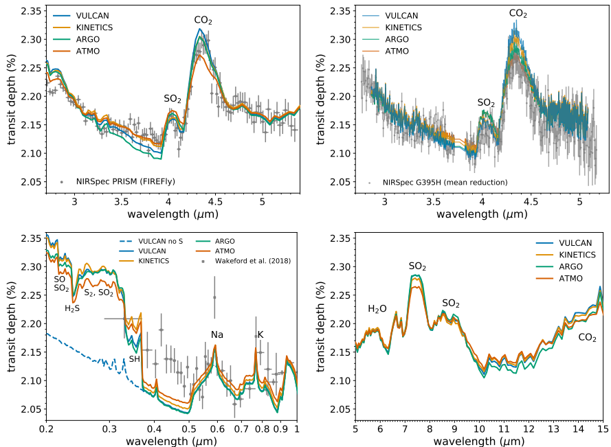
Fig. 3 Morning and evening terminator averaged theoretical transmission spectra generated from 1D photochemical model results. Top left: Comparison to the NIRSpect PRISM FIREFly reduction (Rustankulov et al.(submitted)). Top right: Comparison to the NIRSpect G395H weighted-mean reduction (Alderson et al.(submitted)). Bottom left: Comparison to the current HST and VLT/FORS2 optical wavelength data [20, 21], the models show pronounced features at UV wavelengths due to sulphur species compared to the model without S bearing species (dashed blue line). Bottom right: Predicted spectra across the MIRI LRS wavelength range.
