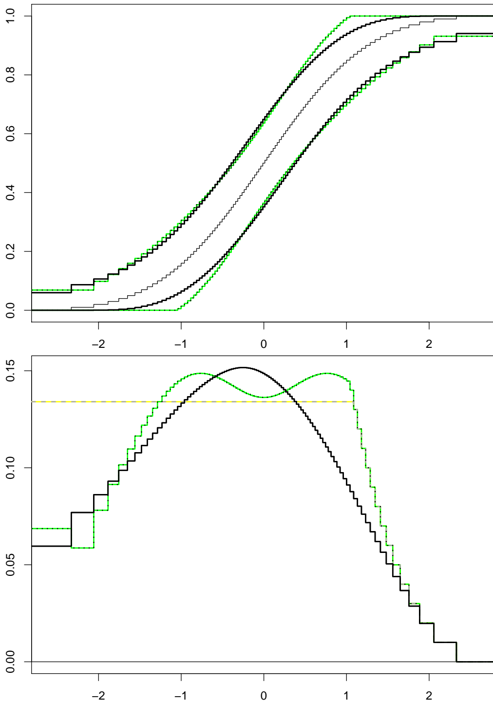
Figure 5: 95%-confidence bands for n = 100 . Upper panel: (A_{n,1,1,\alpha}, B_{n,1,1,\alpha}) (solid) and (A_{n,\alpha}^{\text{SP}}, B_{n,\alpha}^{\text{SP}}) (green, dotted). Lower panel: centered upper bounds B_{n,1,1,\alpha} - \mathbb{F}_n (solid), B_{n,\alpha}^{\text{SP}} - \mathbb{F}_n (green, dotted) and B_{n,\alpha}^{\text{KS}} - \mathbb{F}_n (dashed).
