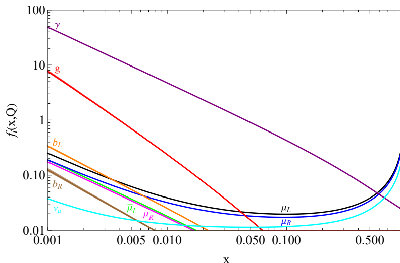
Figure 18. Muon PDFs including the full unbroken SM interactions for Q = 3 \text{ TeV} . The thickness of the gluon and b quarks PDFs is obtained by varying the \mu_{\text{QCD}} scale from 0.5 to 1 GeV.
