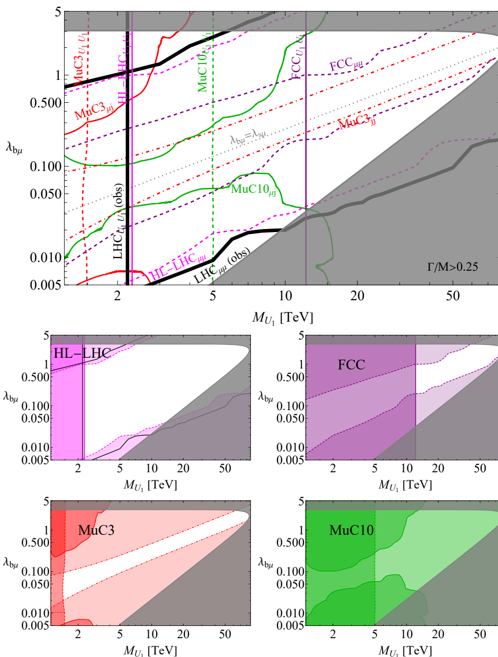
Figure 16. Discovery reach at 5\sigma for the U_1 leptoquark. The fit to bs\mu\mu anomalies is imposed everywhere via eq. (6.6). The present 95%CL exclusion by LHC is shown as a thick black line. The dotted gray line corresponds to \lambda_{b\mu} = \lambda_{s\mu} . In the grey region, the perturbativity criterion \Gamma_{U_1}/M_{U_1} < 0.25 is violated. The limit for the \mu\bar{\mu} \rightarrow jj channel at 10 TeV MuC covers the whole plane. For future colliders, the discoverable region is the one on the side of the line where the corresponding label has been drawn. The smaller figures below the main figure highlight a single future collider at a time.
