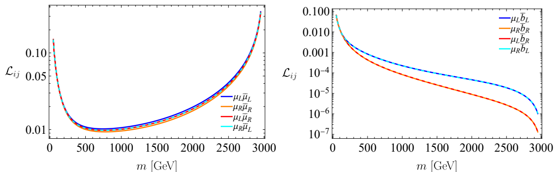
Figure 19. Parton luminosities, for \sqrt{s_0} = 3 \text{ TeV} , involving two muons (left) or a muon and a \bar{b} (right).
