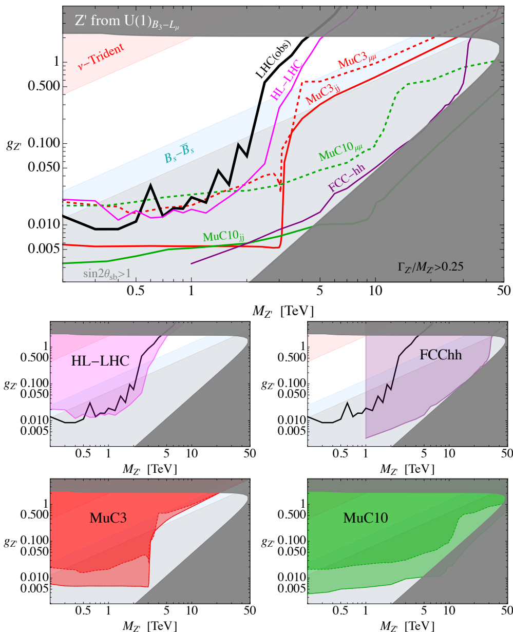
Figure 10. Discovery reach at 5\sigma for the B_3 - L_\mu model. The fit to bs\mu\mu anomalies is imposed everywhere, eq. (5.4). The region excluded at 95% CL by LHC [88] is above the black line, while the one excluded by B_s mixing is colored in light blue. The light gray region cannot provide a successful fit to b \rightarrow s\mu\mu anomalies for values of \sin 2\theta_{sb} < 1 , eq. (5.4), while in the dark gray region the Z' has a large width, signaling a loss of perturbativity. The discoverable region at future colliders is the one on the side of the line where the corresponding label has been drawn. The smaller figures below the main figure highlight a single future collider at a time.
