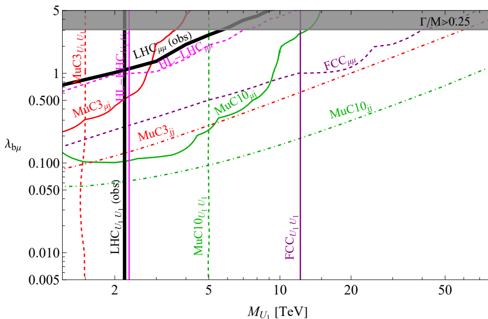
Figure 15. Discovery reach at 5\sigma for the U_1 leptoquark in the U(2)^3 symmetric case. The present 95%CL exclusion by LHC is shown as a thick black line. In the grey region, the perturbativity criterion \Gamma_{U_1}/M_{U_1} < 0.25 is violated.
