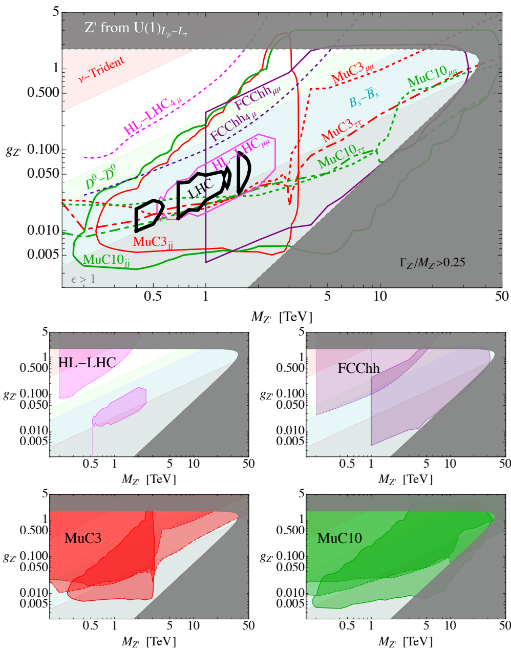
Figure 12. Discovery reach at 5\sigma for the L_\mu - L_\tau model. The fit to bs\mu\mu anomalies is imposed, eq. (5.8). The regions excluded by B_s and D^0 mixings and neutrino trident production are colored in light blue, green and red, respectively. The light gray region requires \epsilon > 1 to fit b \rightarrow s\mu\mu anomalies, while the dark gray region has \Gamma_{Z'}/M_{Z'} > 0.25 . Our recast of the present LHC search [88] excludes at 95% CL the region inside the thick black lines. The discoverable region at future colliders is the one on the side of the line where the corresponding label has been drawn. The smaller figures below the main figure highlight a single future collider at a time.
