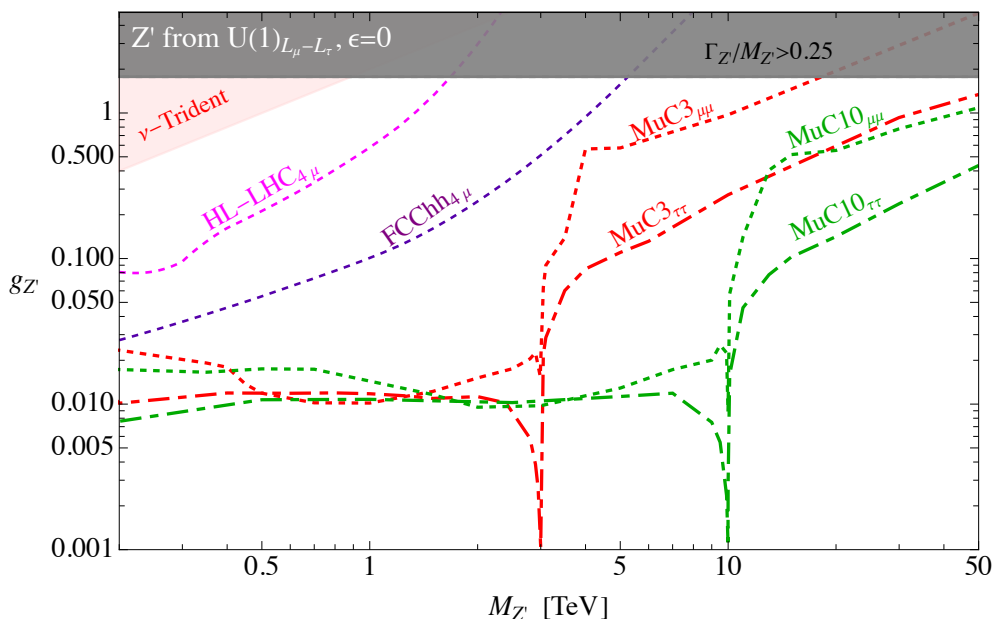
Figure 11. Discovery reach at 5\sigma for the L_\mu - L_\tau model with \epsilon_s = \epsilon_b = 0 in eq. (5.6). In the dark gray region the Z' has a large width, signaling a loss of perturbativity.
