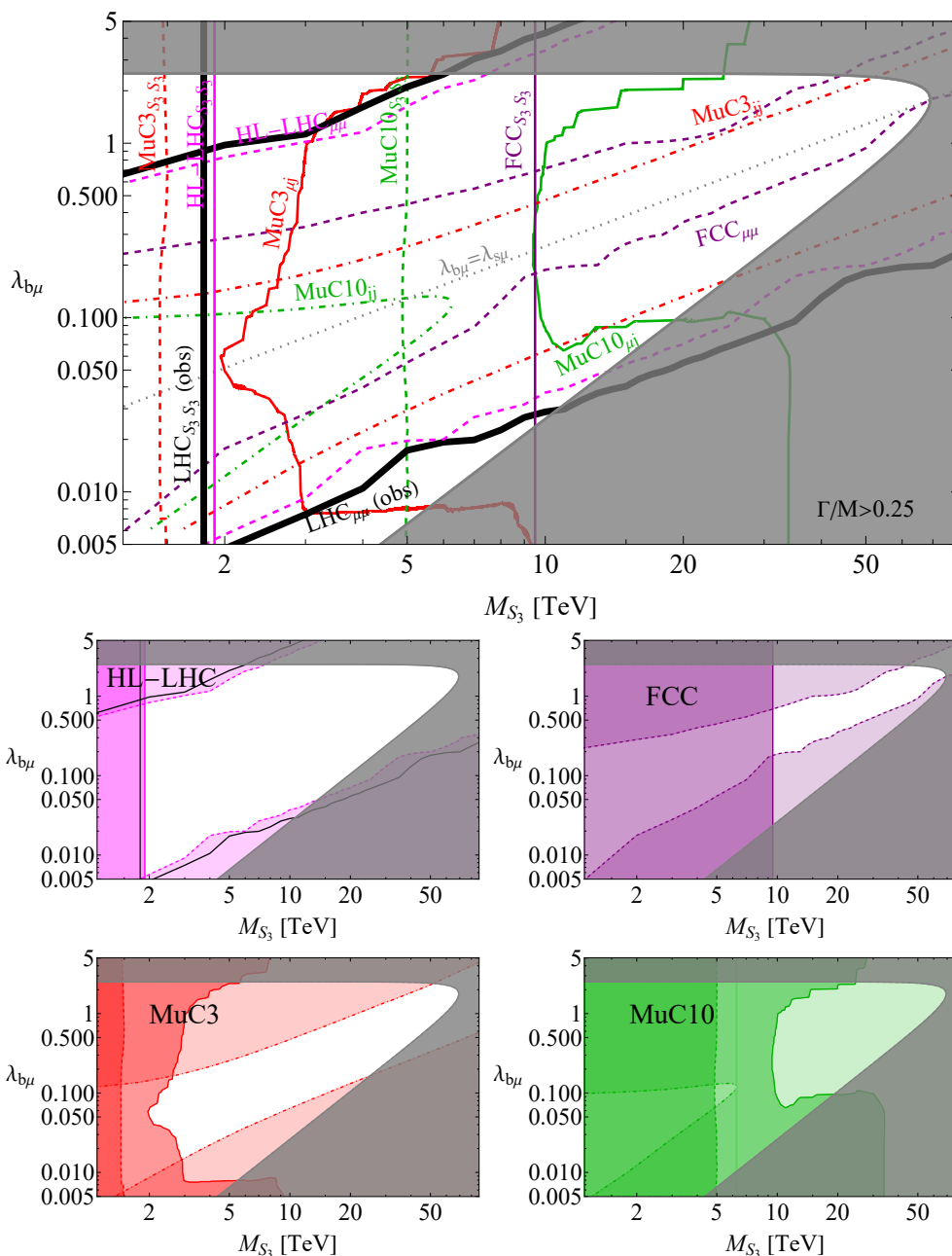
Figure 14. The 5\sigma discovery prospects for the S_3 leptoquark behind to bs\mu\mu anomalies, i.e. imposing eq. (6.6). The present LHC exclusions at 95% CL are shown as a thick black line. The dotted gray line corresponds to \lambda_{b\mu} = \lambda_{s\mu} . The perturbative limit \Gamma_{S_3}/M_{S_3} < 0.25 is violated in the grey region. For future colliders, the discoverable region is on the side of the line where the corresponding label is. The smaller plots below the main one highlight the reach of various future colliders separately.
