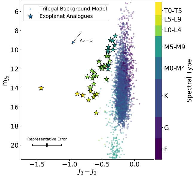
Figure 5. J_3-J_2 versus m_{J_3} colour-magnitude diagram. Young, late-type exoplanet analogues (stars) are plotted, as well objects returned for Trilegal Galactic model along the \beta Pictoris line of sight are plotted (circles), with the point colour indicating the spectral type of each object. Representative error bar from SHINE F150 shown in bottom left. The arrow plotted shows the A_V = 5 extinction vector.
