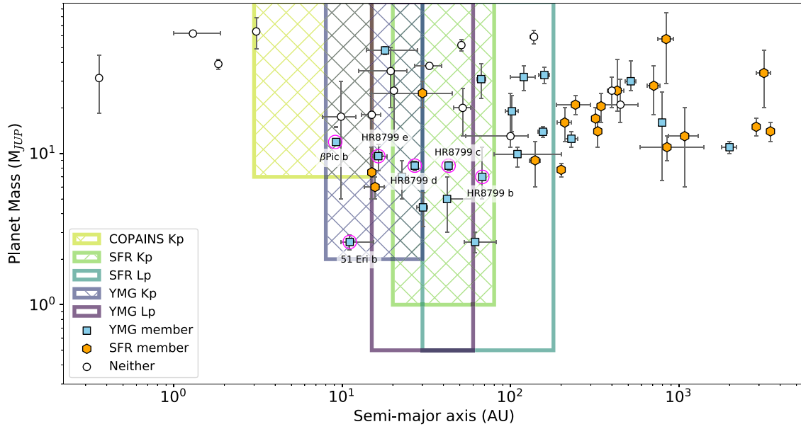
Figure 10. Planet mass versus semimajor axis. Plotted are planets and brown dwarfs detected using direct imaging (exoplanet.eu). Colour-coding of points indicates members of young moving groups (blue) or star-forming regions (orange). Rectangular regions show the possible sensitivities for each survey approach. Cross-hatched areas indicate NIX simulations using the K -peak filter, areas with no fill are NIX simulations using the L filter.
