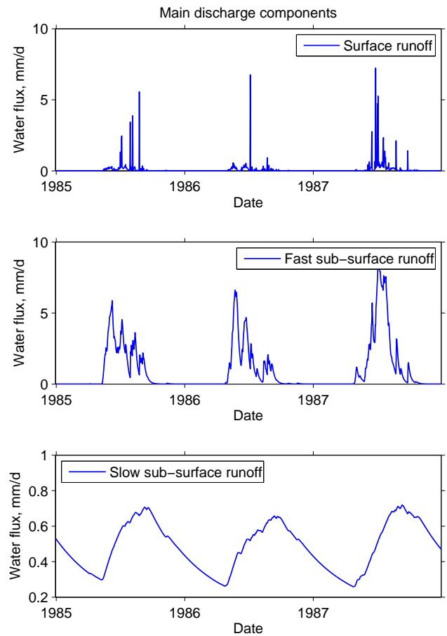
Figure 5. Time series of the streamflow components (direct surface flow, fast subsurface flow and slow (deep) subsurface flow) corresponding to the parameter set of Table 3 and the discharge plot of Fig. 4.
