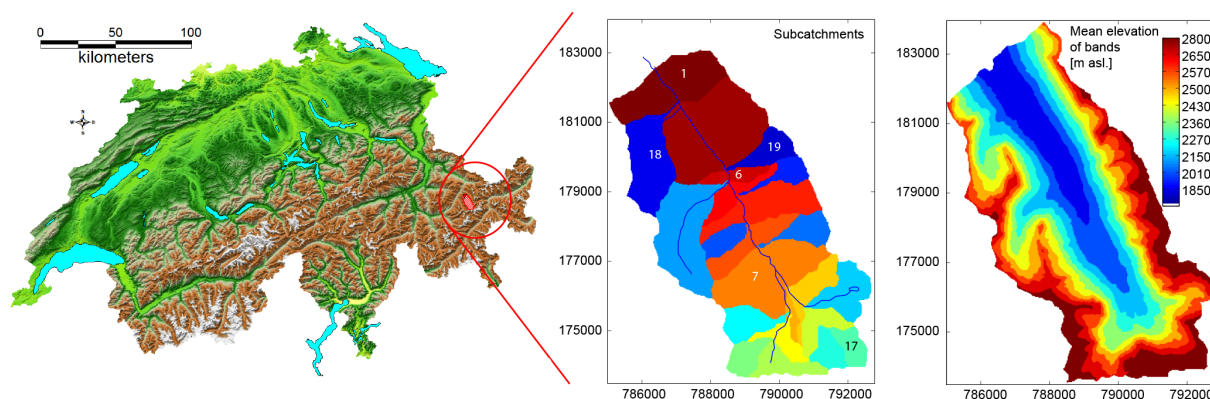
Figure 3. Location of the Dischmabach catchment within Switzerland (source: SwissTopo, 2005, 2008) and the 23 subcatchments identified with TauDEM Version 5 (Tarboton, 1997). The 10 elevation bands in the right plot are used for comparison purposes in Sect. 5.1. The latitude and longitude are indicated in the Swiss coordinate system (in km).
