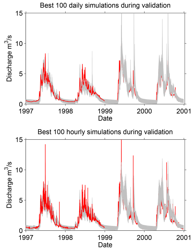
Figure 7. Predictions resulting from the 100 best parameter sets obtained under NSE for a daily time step (of the total 35 000 Monte Carlo simulations); top: simulation at the daily time step, bottom: simulation at the hourly time step (same parameter sets). The first half of the plot shows that the prediction limits are reasonably narrow, the reserved plotting order in the second half shows that the observations are well spanned – 79 % (daily) respectively 75 % (hourly) of the observed time steps fall into the range spanned by the simulations.
