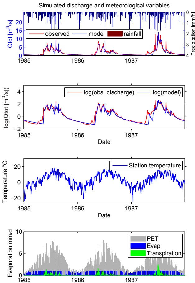
Figure 4. Observed and simulated hydro-meteorological time series of model state variables for the parameter set of Table 3.
