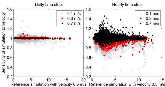
Figure 9. Sensitivity of the discharge simulation with respect to the in-stream flow velocity plotted against the reference simulation with parameters of Table 3 and velocity of 0.5 \text{ m s}^{-1} ; the sensitivity is expressed as the relative difference to the reference simulation for each time step.
