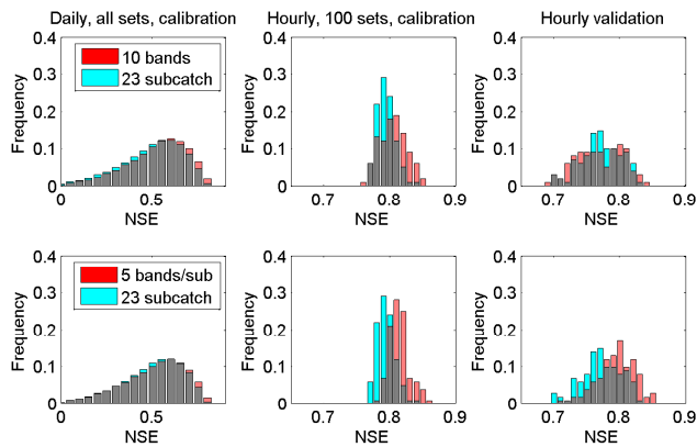
Figure 10. Comparison of model performance of the subcatchment-based model set-up (23 subcatchments) to elevation band set-ups. Top row: comparison to 10 elevation bands (see Fig. 3), bottom row: comparison to a combination of elevation bands and subcatchments (5 bands for each of the 23 subcatchments). Left column: distribution of the Nash–Sutcliffe (NSE) efficiency computed at a daily time step for the calibration period (shown are parameter sets with \text{NSE} > 0 ); centre column: NSE distribution of the 100 sets with the highest NSE values at the daily time step run at hourly time step for the calibration period; right column: same 100 sets run at an hourly time step for the validation period. The same 35 000 parameter sets are run for all three model set-ups.
