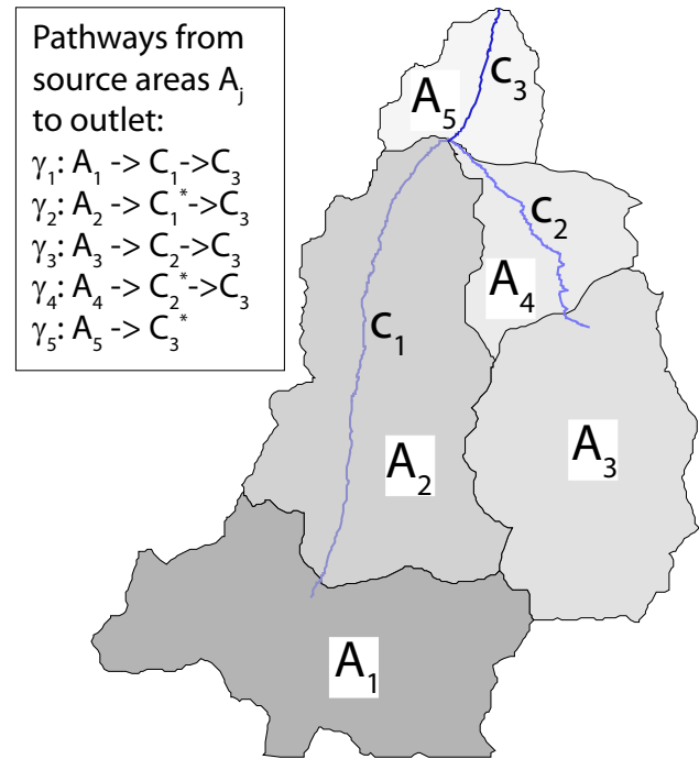
Figure 2. Sketch of the flow paths from a catchment with five source areas A_j and three channels C_j . The notation C_j^* means that the injection into this channel is not concentrated at the upstream end but, in theory, randomized and integrated over the channel length (Bras and Rodriguez-Iturbe, 1985). In practice, we take half of the channel length.
