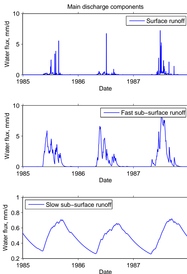
Figure 5. Time series of the streamflow components (direct surface flow, fast subsurface flow and slow (deep) subsurface flow) corresponding to the parameter set of Table 3 and the discharge plot of Fig. 4.
