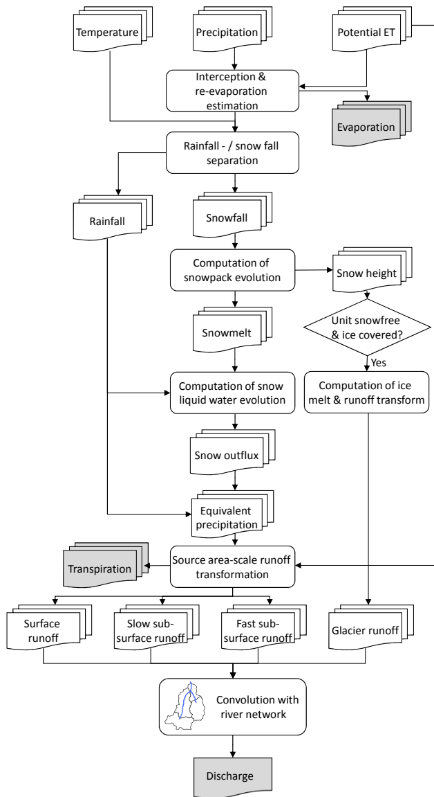
Figure 1. Flow diagram of the precipitation–discharge computation. The grey boxes highlight the model output time series.
