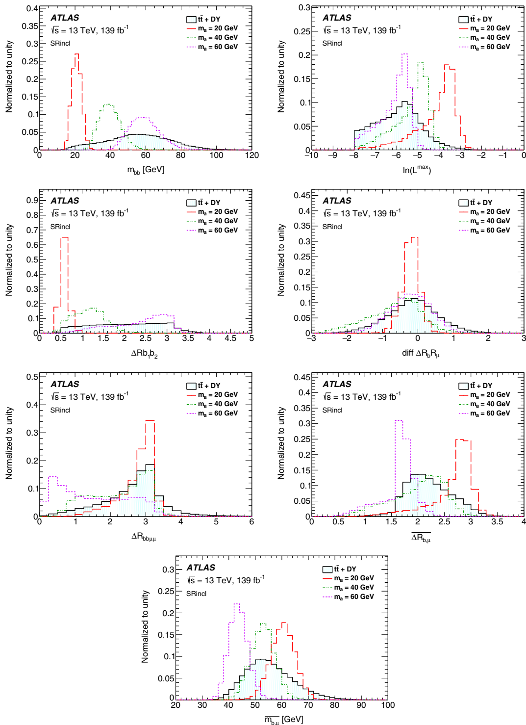
FIG. 1. Kinematic variables used as inputs to the BDT training. From top left to bottom right: m_{bb} , \ln(L^{\max}) , \Delta R_{b_1 b_2} , \text{diff} \Delta R_{b_1 R_\mu} , \Delta R_{bb\mu\mu} , \overline{\Delta R_{b,\mu}} , \overline{m_{b,\mu}} . The variables are plotted in SRincl. All the distributions are normalized to unit area. The background histogram is the sum of the t\bar{t} and DY event templates, combined in the proportions extracted from the background validation fit described in Sec. VII.
