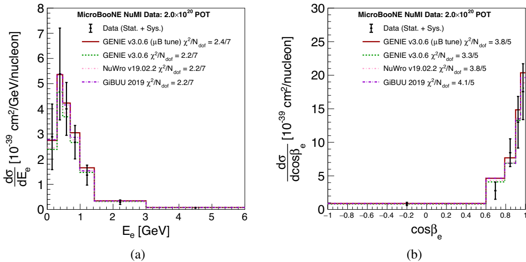
FIG. 2. Unfolded differential cross section as a function of the electron (a) energy and (b) angle. The data cross section is compared to GENIE v3.0.6 ( \mu B tune)(red), GENIE v3.0.6 (green), NuWro v19.02.2 (pink), and GiBUU 2019 (purple), and is in agreement with all predictions.
