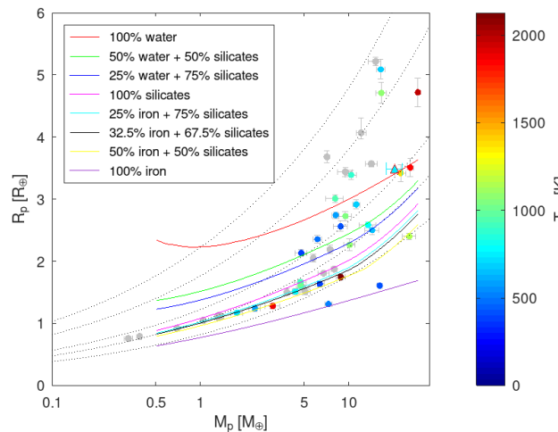
Fig. 3. Mass-radius diagram showing exoplanets with M_p < 30 M_\oplus , whose estimated mean density \rho_p is more precise than 15%. TOI-1055 b is represented by a triangle. All markers are colour-coded according to the planetary equilibrium temperature, T_{\text{eq}} , where available. Dotted black lines represent the loci of constant \rho_p equal to 0.5, 1, 3, 5, and 10 g cm -3 (from top to bottom). Solid lines represent different planet composition models (as explained in the legend) computed for an equilibrium temperature T_{\text{eq}} = T_{\text{eq,TOI-1055b}} = 750 K.
