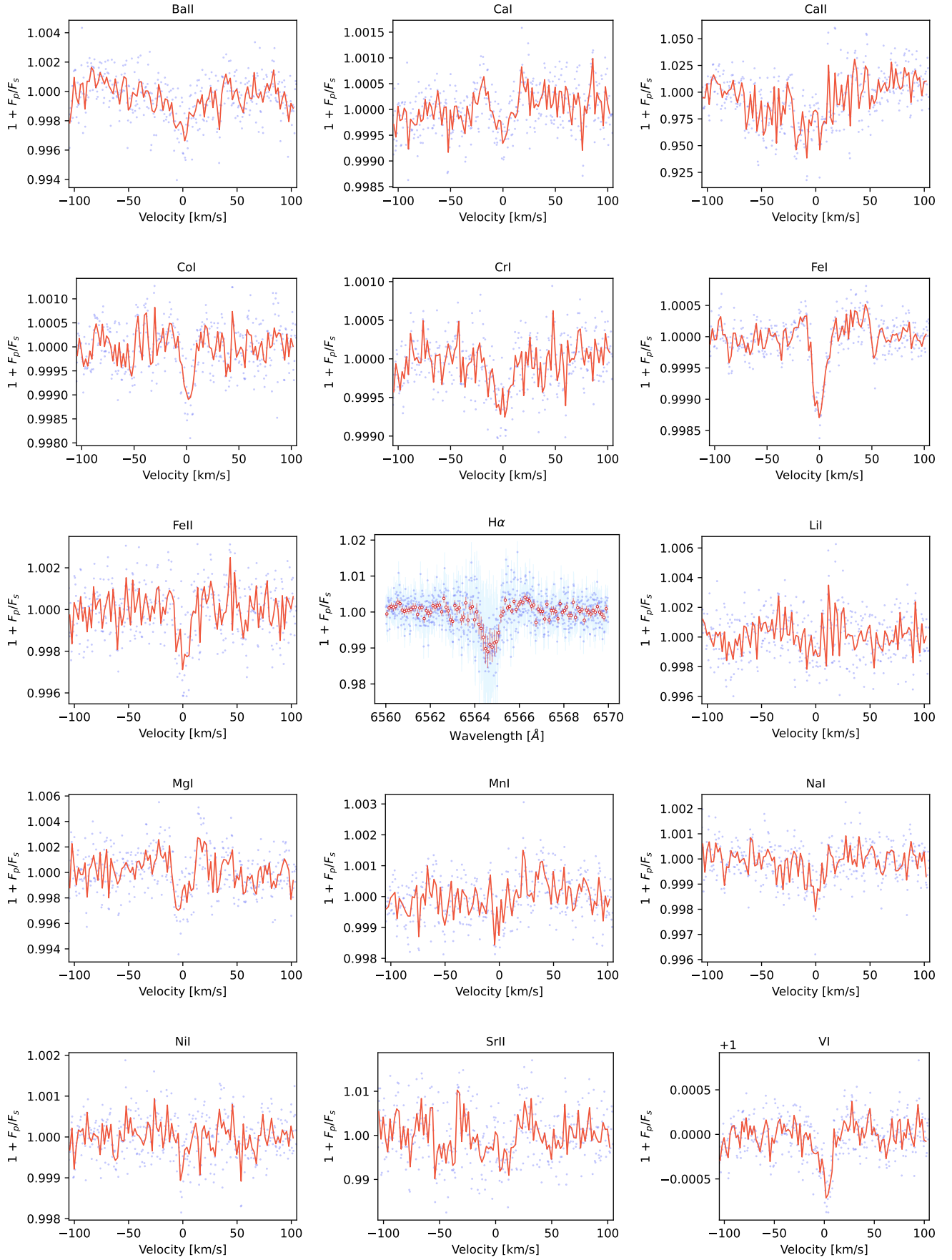
Fig. H.5. Same as Fig. H.1 for WASP-121b, night 1 (UT - 2018 November 30).
