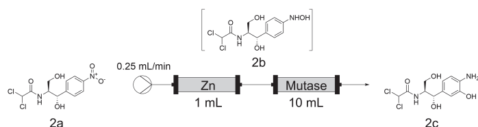
Fig. 2. Transformation of chloramphenicol ( 2a ) (1 mM) into ortho -amino-phenol derivative ( 2c ). [8]
