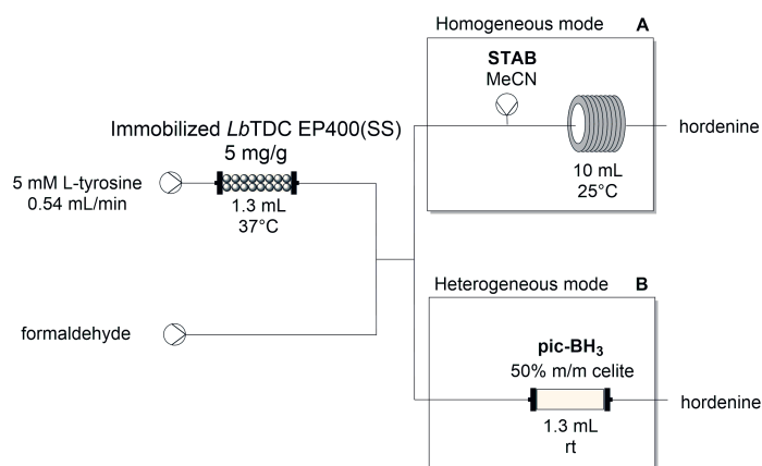
Fig. 9. Alkylation of tyramine with formaldehyde and reducing agent.
