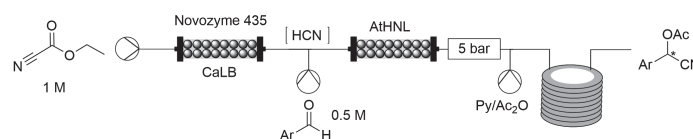
Fig. 4. Three-step continuous chemoenzymatic cascade towards chiral O-acetylcyanohydrins.
