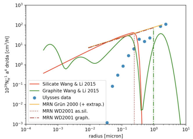
Figure 2. The ISD mass distribution from astronomical models and in situ data by Ulysses. Most of the mass is in the largest particles, which is important for the determination of the gas-to-dust mass ratio. Units on the vertical axis are chosen to be equal to the units in Wang et al. (2015). Distributions derived from astronomical observations were taken from Wang et al. (2015), Grün & Landgraf (2000), Weingartner & Draine (2001). Ulysses data are from Krüger et al. (2015).
