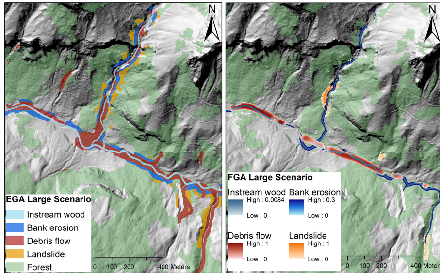
Figure 4. Large-scenario comparison of model outputs from the EGA (left) and FGA (right) at the Spiggebach torrent within the Chiene river catchment (canton of Bern). Potential recruitment areas are shown for landslides (orange), debris flows (red), and bank erosion (dark blue). The stream network (light blue) also includes instream wood loads. Background: digital terrain model (hillshade), © swisstopo.
