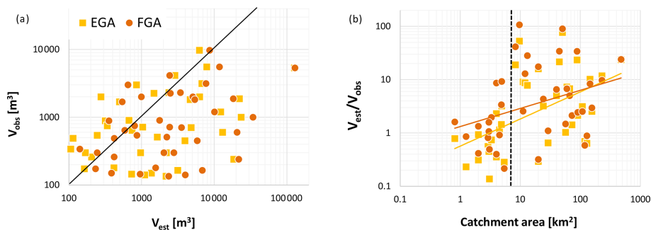
Figure 9. (a) Modelled LW V_{\text{est}} (large scenario) versus observed wood volume V_{\text{obs}} during past events. The black line shows the line of equality (1 : 1 line). (b) Ratio of V_{\text{est}}/V_{\text{obs}} versus catchment area.
