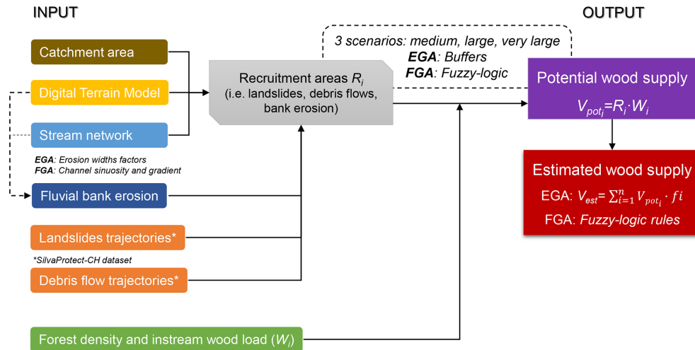
Figure 1. Conceptual model of the empirical GIS approach (EGA) and the fuzzy-logic GIS approach (FGA). V_{pot} : potential wood supply [ m^3 ]; V_{est} : estimated supplied wood [ m^3 ]; i : recruitment process [-]; R : recruitment area [ha]; W : forest density or instream wood load [ m^3 ha^{-1} ]; f : volume reduction factor [-]. Three different scenarios were defined (see Sect. 3.5): medium scenario (medium to high frequency and intermediate magnitude), large scenario (relatively low frequency and medium to high magnitude), and very large scenario (very low frequency and very high magnitude).
