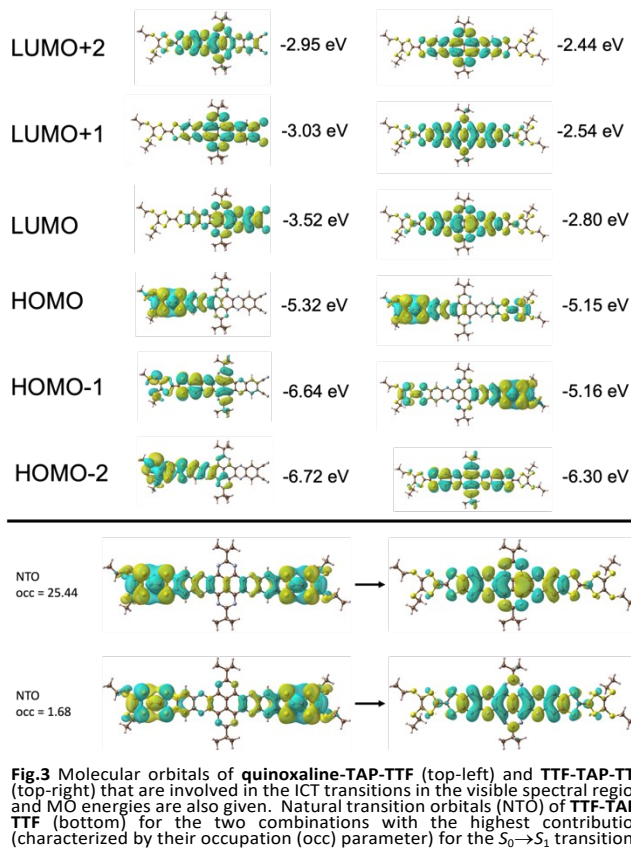
Fig. 3 Molecular orbitals of quinoxaline-TAP-TTF (top-left) and TTF-TAP-TTF (top-right) that are involved in the ICT transitions in the visible spectral region and MO energies are also given. Natural transition orbitals (NTO) of TTF-TAP-TTF (bottom) for the two combinations with the highest contribution (characterized by their occupation (occ) parameter) for the S_0 \rightarrow S_1 transition.
