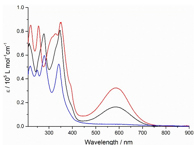
Fig. 1 The UV-Vis absorption spectra of quinoxaline-TAP-TTF (black), TTF-TAP-TTF (red) and diquinoxaline-TAP (blue) ( c = 5 \times 10^{-6} M) in THF at r.t.
