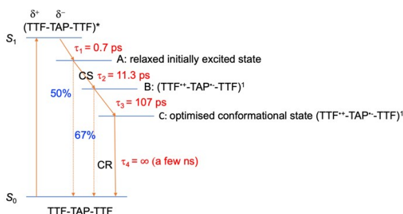
Fig. 6 Schematic representation of the relaxation processes for TTF-TAP-TTF upon excitation at 580 nm into the ICT band. A: relaxed initially excited state, B: singlet charge-separated state, C: optimised conformational singlet charge-separated state.
