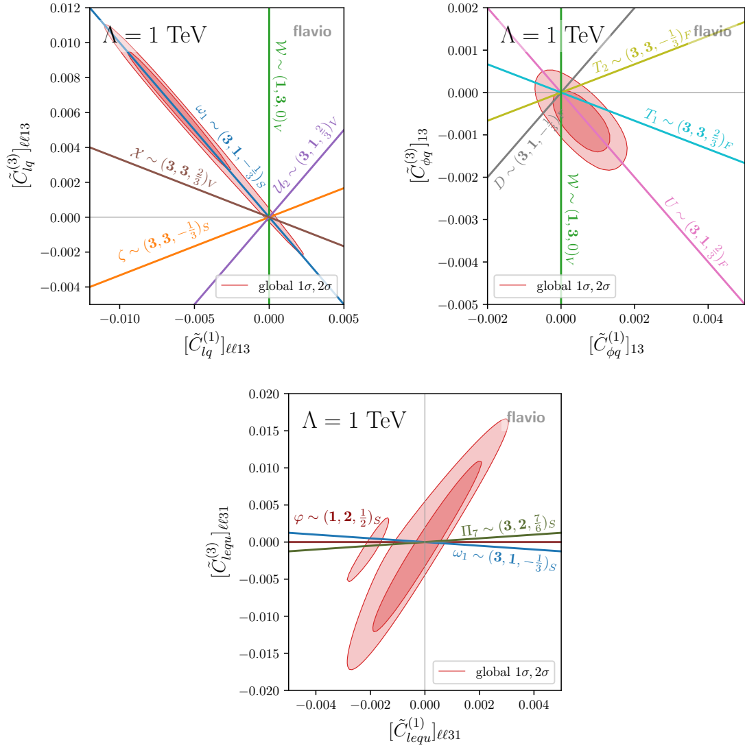
Figure 7. The 1σ and 2σ contours of a global SMEFT fit overlaid with directions generated by single-mediator tree-level models in the scenarios ([\tilde{C}_{lq}^{(1)}]_{\ell\ell 13}, [\tilde{C}_{lq}^{(3)}]_{\ell\ell 13}) , ([\tilde{C}_{\phi q}^{(1)}]_{13}, [\tilde{C}_{\phi q}^{(3)}]_{13}) , and ([\tilde{C}_{lequ}^{(1)}]_{\ell\ell 31}, [\tilde{C}_{lequ}^{(3)}]_{\ell\ell 31}) . See text for detailed discussion.
