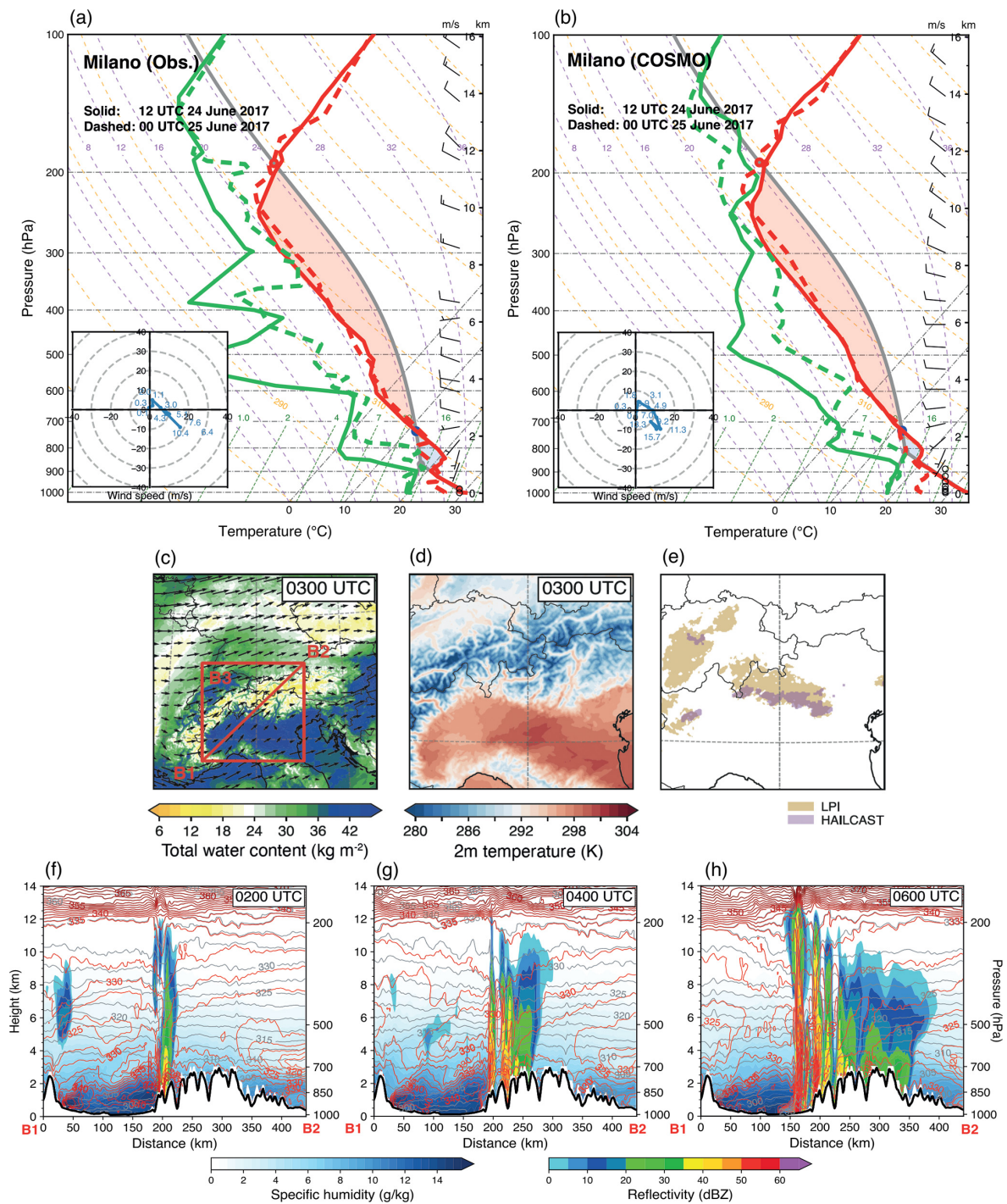
Figure 11. As in Fig. 10, but for the case of 25 June 2017. (a) Sounding observations and (b) COSMO extracted profiles at Milano at 12:00 UTC on 24 June 2017 (solid lines) and 00:00 UTC on 25 June 2017 (dashed lines). (c) COSMO simulated total water content and vertically integrated water flux vectors, (d) 2m temperature at 03:00 UTC on 25 June 2017, and (e) footprints of LPI and HAILCAST obtained between 03:00 and 04:00 UTC are shaded in yellow and purple, respectively. The red box B3 in (c) indicates the zoomed subdomain shown in (d, e) . (f–h) Vertical cross sections of potential temperature (gray contours), equivalent potential temperature (red contours), specific humidity (blue shaded), and simulated reflectivity (color shaded) along the red transect B1–B2 at 02:00, 04:00, and 06:00 UTC on 25 June 2017.
