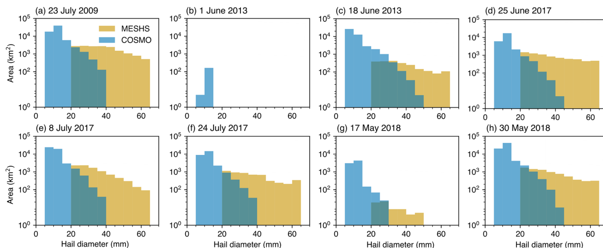
Figure 6. Area affected by hail obtained in radar-based MESHS observations (orange) and COSMO HAILCAST (blue) for all eight cases analyzed over the radar domain (Fig. 1). Note that MESHS estimates are only available for diameters > 20 mm.
