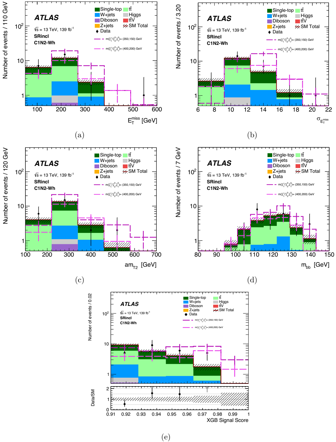
Figure 8. Post-fit distributions in the SRs (not binned in signal output score) for representative kinematic observables (a) E_T^{\text{miss}} , (b) \sigma_{E_T^{\text{miss}}} , (c) am_{T2} , (d) m_{b\bar{b}} and (e) the signal output score. Two representative SUSY signal models are overlaid for illustration. The uncertainty bands plotted include all statistical and systematic uncertainties. The overflow events, where present, are included in the last bin.
