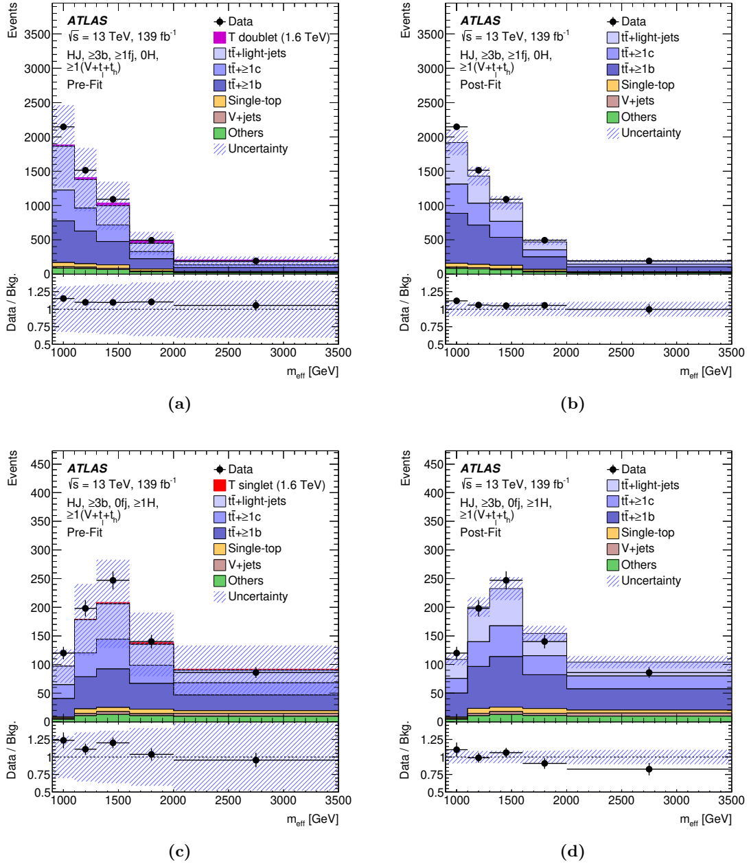
Figure 10. Comparison between the data and prediction for the m_{\text{eff}} distribution under the background-only hypothesis, in the (HJ, \geq 3b, \geq 1f_j, 0H, \geq 1(V+t_l+t_h)) validation region (a) pre-fit and (b) post-fit, and the (HJ, \geq 3b, 0f_j, \geq 1H, \geq 1(V+t_l+t_h)) validation region (c) pre-fit and (d) post-fit. The expected T doublet signal (solid purple) for m_T = 1.6 TeV and \kappa = 0.5 is included in the pre-fit figures. The “others” background includes the t\bar{t} V/H , VH , tZ , t\bar{t}t\bar{t} , diboson, and multijet backgrounds. The bottom panels display the ratios of data to the total background prediction. The hashed area represents the total uncertainty in the background. The last bin in each distribution contains the overflow.
