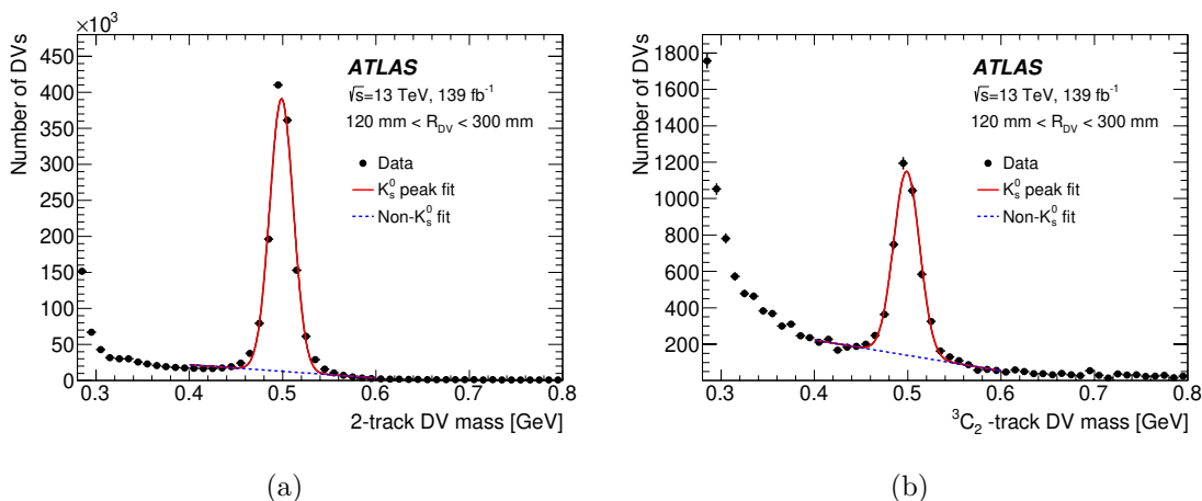
Figure 7. The mass spectrum of preselected (a) 2-track DVs and (b) 2-track combinations of 3-track DVs ( {}^3\text{C}_2 ) in one radial region. The mass spectrum is fit to a Gaussian function centered on the K_S^0 mass and a linear background. The data in the K_S^0 mass spectrum after subtracting the fitted background is used to compute the K_S^0 crossing factors.
