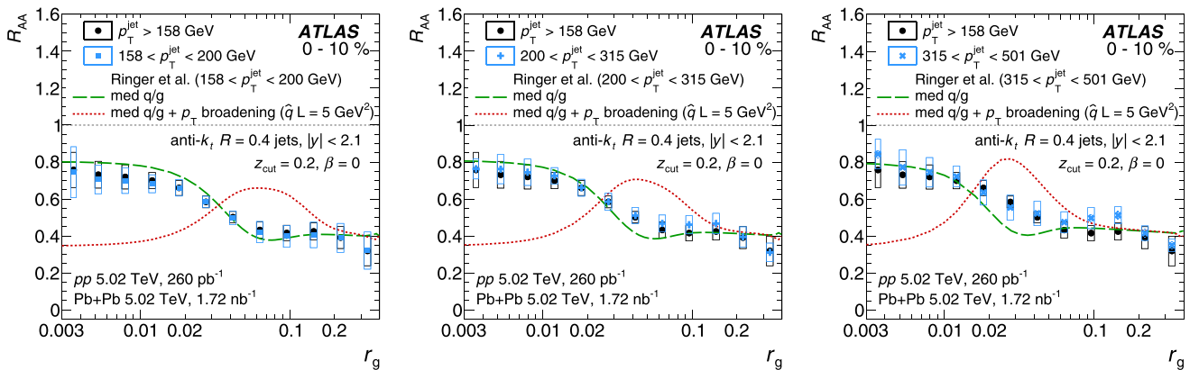
FIG. 14. Comparison of R_{AA} as a function of r_g for three intervals of p_T^{\text{jet}} in 0–10% centrality Pb+Pb events with theoretical predictions from Ringer et al. [93]. The error bars and the open boxes around the data points represent the statistical and systematic uncertainties, respectively. The uncertainties in the pp luminosity (1.6%) and \langle T_{AA} \rangle are not included, but are listed in Table I. The green curve (med q/g) represents the quark and gluon differential energy loss setting. The red curve (med q/g + p_T broadening) adds transverse momentum broadening effects for all subjects in the medium.
