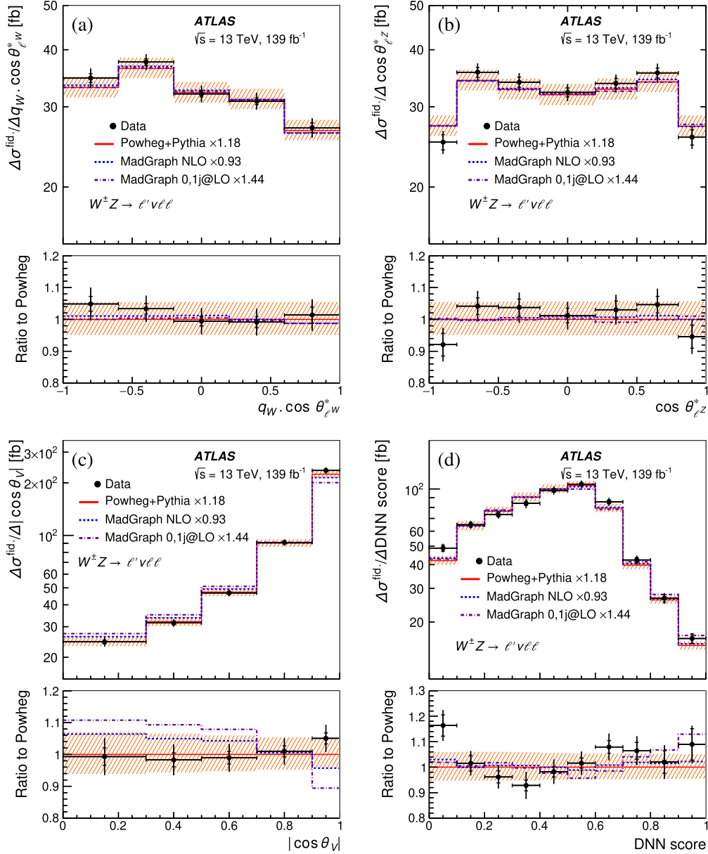
Fig. 5. The measured W^\pm Z differential cross section in the fiducial phase space as a function of (a) q_W \cdot \cos\theta_{\ell W}^* , (b) \cos\theta_{\ell Z}^* , (c) |\cos\theta_V| and (d) DNN score. The total cross section integrated over each bin and divided by the bin width is represented. The inner and outer error bars on the data points represent the statistical and total uncertainties, respectively. The measurements are compared with the NLO prediction from POWHEG+PYTHIA (solid line). The dashed band shows how the sum of QCD scale and PDF uncertainties affects the POWHEG+PYTHIA prediction. The predictions from the MADGRAPH 0,1j@LO and MADGRAPH5_AMC@NLO+PYTHIA MC generators are also indicated by dotted-dashed and dashed lines, respectively. All predictions have been scaled to the NNLO QCD integrated cross section predicted by MATRIX.
