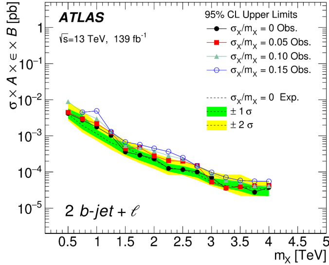
(b) Limits for m_{bb\ell}
