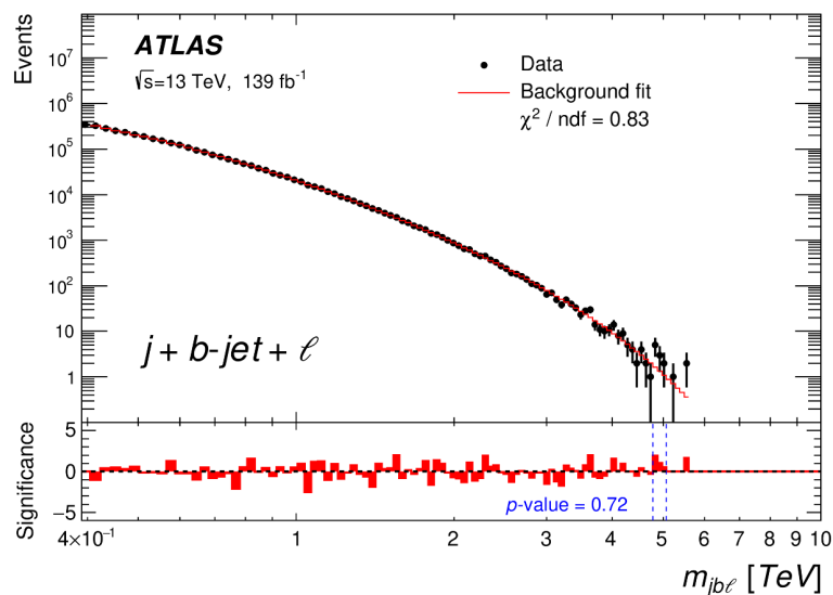
(a) m_{jbl} invariant mass
