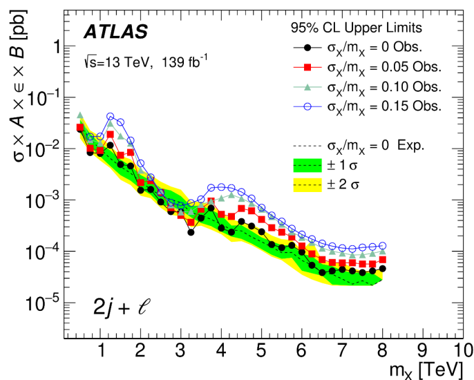
Figure 6. The 95% CL observed upper limits, in the m_{jj\ell} channel, on the cross-section times acceptance ( A ), efficiency ( \epsilon ) and branching ratio ( B ) for a Gaussian signal with various signal widths. The expected limit and the corresponding \pm 1\sigma and \pm 2\sigma bands are shown for \sigma_X/m_X = 0 signals. The limit for a width of 15% is shown starting from 0.75 TeV in order to avoid the region close to the minimum value of the m_{jj\ell} distribution.
