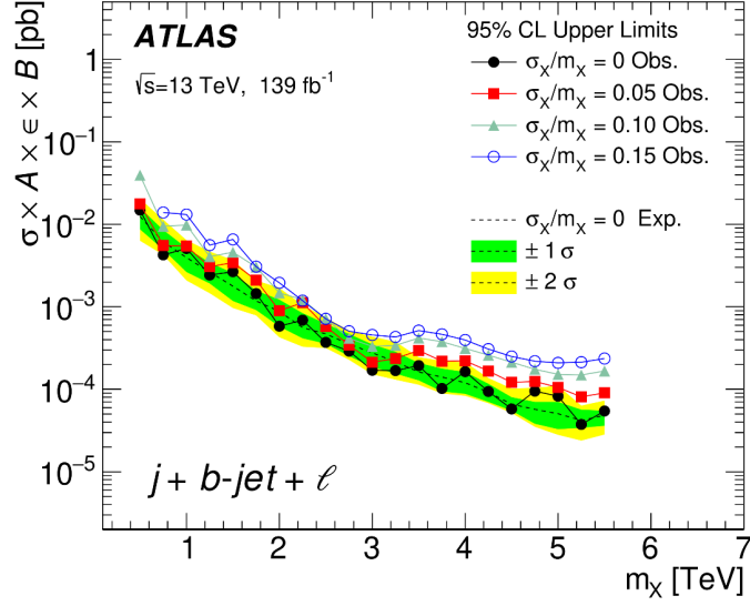
(a) Limits for m_{jbl}
