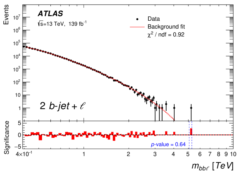
(b) m_{bbell} invariant mass
