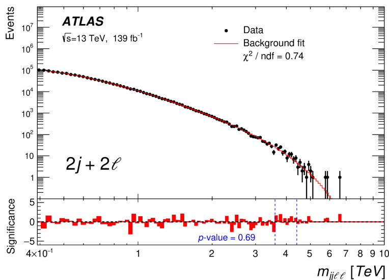
Figure 4. Invariant 2j + 2\ell mass distribution for m_{jj\ell\ell} > 0.4 TeV together with the fit with the 5p background function. The lower panel shows the bin-by-bin significances of deviations from the background hypothesis. The largest deviation reported by the BumpHunter algorithm is shown by the vertical dashed lines. The global p -value of this deviation in the range 3.59–4.41 TeV is indicated.
