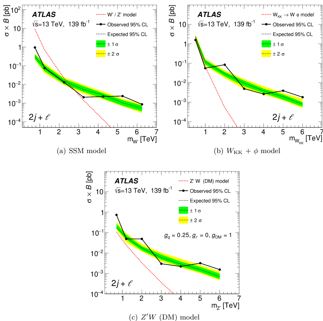
Figure 9. Observed (filled circles) and expected (dotted line with uncertainty bands) 95% CL upper limits on the cross-section ( \sigma ) times branching ratio ( B ) for (a) the SSM W' boson, (b) the W_{KK} + \phi radion model with m_{W_{KK}} - m_{\phi} = 250 GeV, and (c) the Z'W simplified DM model. The presented limits were obtained using the m_{jj\ell} ( \ell = \mu, e ) distribution in events with at least one isolated lepton with p_T^{\ell} > 60 GeV. Branching ratios of 100% to the final states of interest were assumed in the signal generation and computation of theory cross-sections. The black lines shown for the observed limits are provided to guide the eye.
