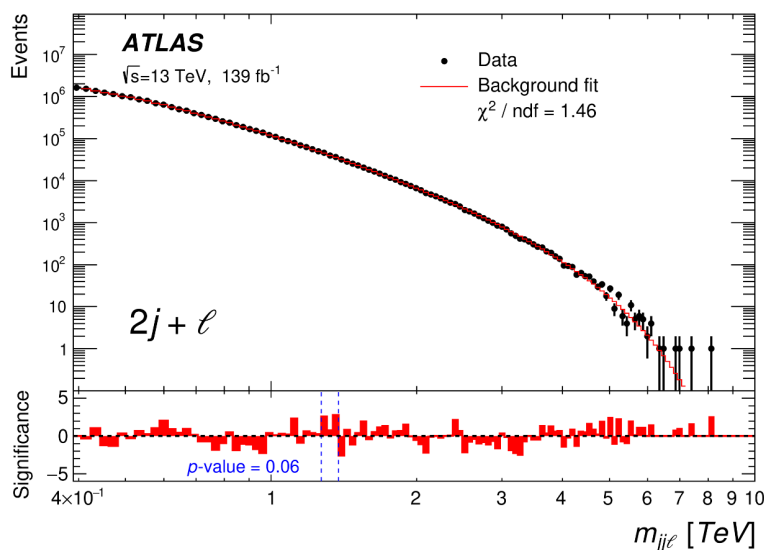
Figure 3. Invariant 2j + \ell mass distribution for m_{jj\ell} > 0.4 TeV together with the fit with the 5p background function. The lower panel shows the bin-by-bin significances of deviations from the background hypothesis. The largest deviation reported by the BumpHunter algorithm is shown by the vertical dashed lines. The global p -value of this deviation in the range 1.27–1.38 TeV is indicated.
