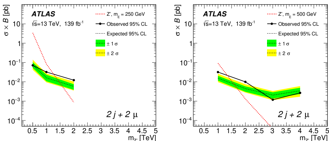
(a) Composite-lepton model with m_E = 250 GeV (b) Composite-lepton model with m_E = 500 GeV
