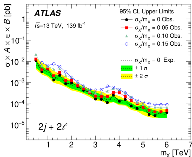
Figure 7. The 95% CL observed upper limits, in the m_{jj\ell\ell} channel, on the cross-section times acceptance ( A ), efficiency ( \epsilon ) and branching ratio ( B ) for a Gaussian signal with various signal widths. The expected limit and the corresponding \pm 1\sigma and \pm 2\sigma bands are shown for \sigma_X/m_X = 0 signals. The limit for a width of 15% is shown starting from 0.75 TeV in order to avoid the region close to the minimum value of the m_{jj\ell\ell} distribution.
