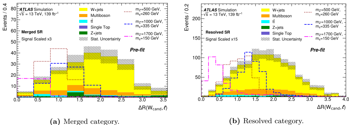
Figure 5. Distributions of \Delta R(W_{\text{cand}}, \ell) in the signal region for the merged (a) and resolved (b) category, before any fit (‘Pre-fit’). The contributions from all SM backgrounds are shown as a histogram stack. The ‘multiboson’ category includes contributions from VV , VVV , and electroweak VVjj production. The hatched bands represent the total MC statistical uncertainty of the SM expectation. The expected signal from a representative set of dark Higgs models with g_q = 0.25 , g_\chi = 1 , m_\chi = 200 \text{ GeV} , and \sin \theta = 0.01 scaled for presentation purposes is also shown for reference. All selection criteria for the corresponding category (see tables 2 and 3) are applied, except the one for the displayed observable.
