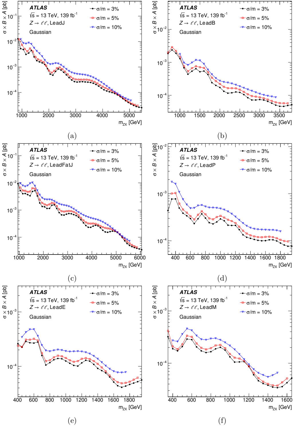
Figure 10. Comparison of observed upper limits at 95% CL on the cross section times branching fraction times acceptance for a Gaussian-shaped signals with relative width values of 3%, 5% and 10% as a function of m_{ZX} in the (a) leading small- R -jet, (b) leading b -jet, (c) leading large- R -jet, (d) leading photon, (e) leading electron, and (f) leading muon categories.
