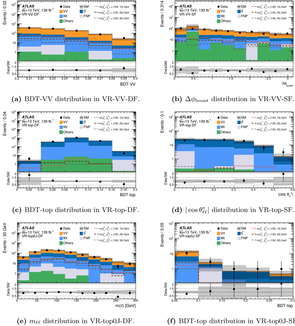
Figure 4. Distributions of (a) BDT-VV in VR-VV-DF, (b) \Delta\phi_{\text{boost}} in VR-VV-SF, (c) BDT-top in VR-top-DF, (d) |\cos\theta_{\ell\ell}^*| in VR-top-SF, (e) m_{\ell\ell} in VR-top0J-DF and (f) BDT-top in VR-top0J-SF, for data and the estimated SM backgrounds. The normalization factors extracted from the corresponding CRs are used to rescale the t\bar{t} , single-top-quark and VV backgrounds. The FNP lepton background is calculated using the data-driven matrix method. ‘Others’ include the non-dominant background sources, e.g. t\bar{t}+V , Higgs boson and Drell-Yan events. The uncertainty band includes systematic and statistical errors from all sources and the last bin includes the overflow. Distributions for three benchmark signal points are overlaid for comparison. The lower panels show the ratio of data to the SM background estimate.
