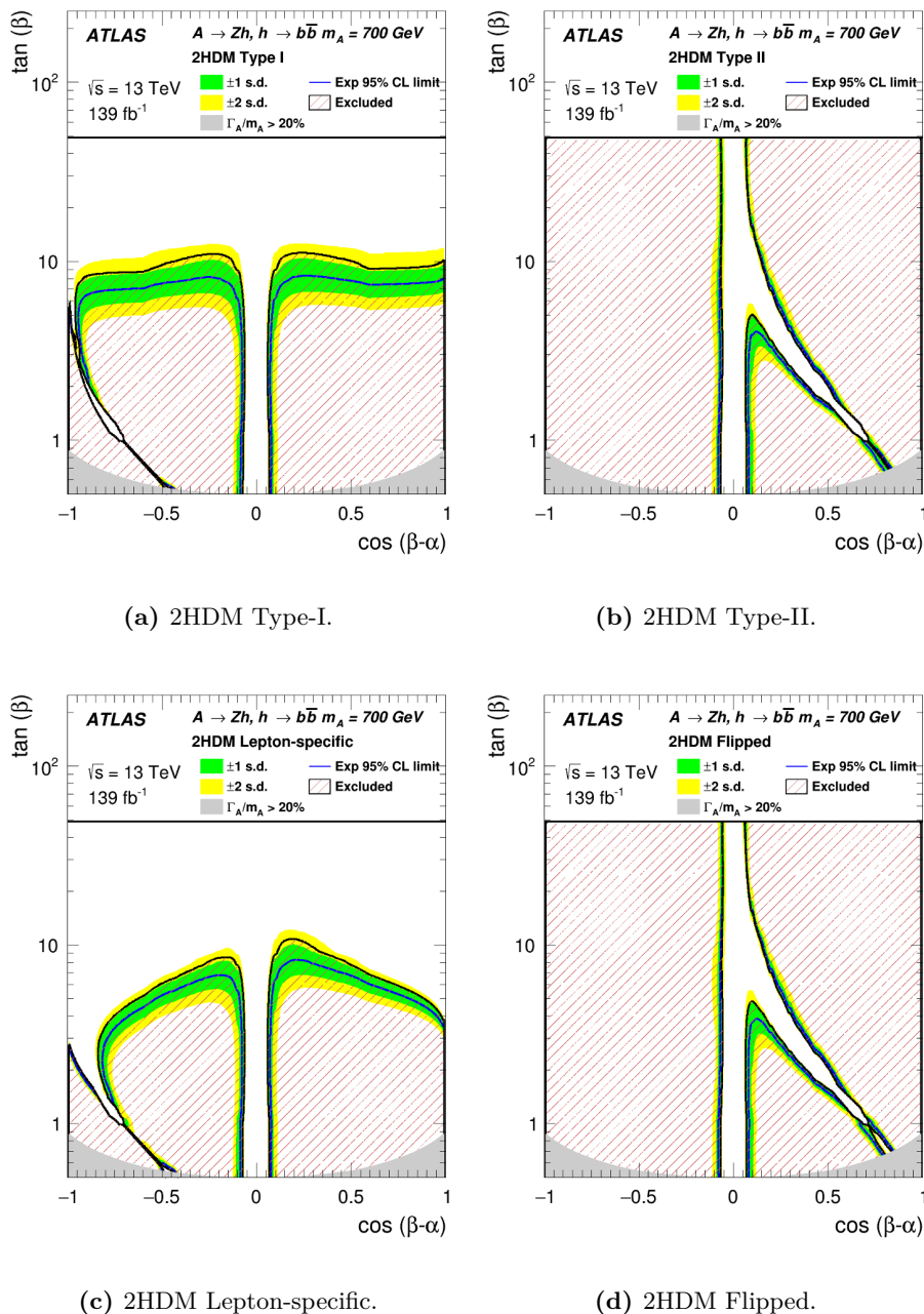
Figure 12. The interpretation of the cross-section limits in the context of the various 2HDM types as a function of the parameters \tan \beta and \cos(\beta - \alpha) for m_A = 700 GeV: (a) Type-I , (b) Type-II, (c) Lepton-specific, and (d) Flipped. Variations of the natural width up to \Gamma_A/m_A = 20\% have been taken into account. For the interpretation in Type-II and Flipped 2HDM, the b -quark associated production is included in addition to the gluon-gluon fusion production. The exclusion limits are only evaluated for \tan \beta < 50 because larger \tan \beta values are disfavoured by most models (and cross-section predictions become less reliable).
